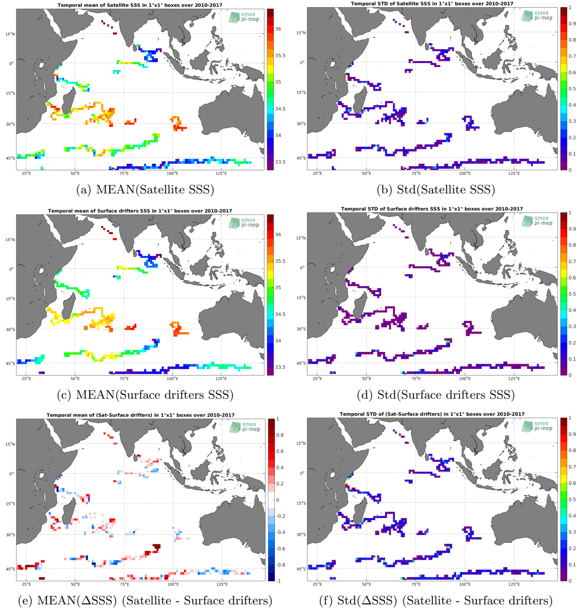
Figure 5: Temporal mean (left) and Std (right) of SSS from SMOS-L3-CATDS-CECOS-LOCEAN-V3-9DAYS-25KM (top), Surface drifters (middle), and of \Delta SSS (Satellite - Surface drifters). Only match-up pairs are used to generate these maps.
