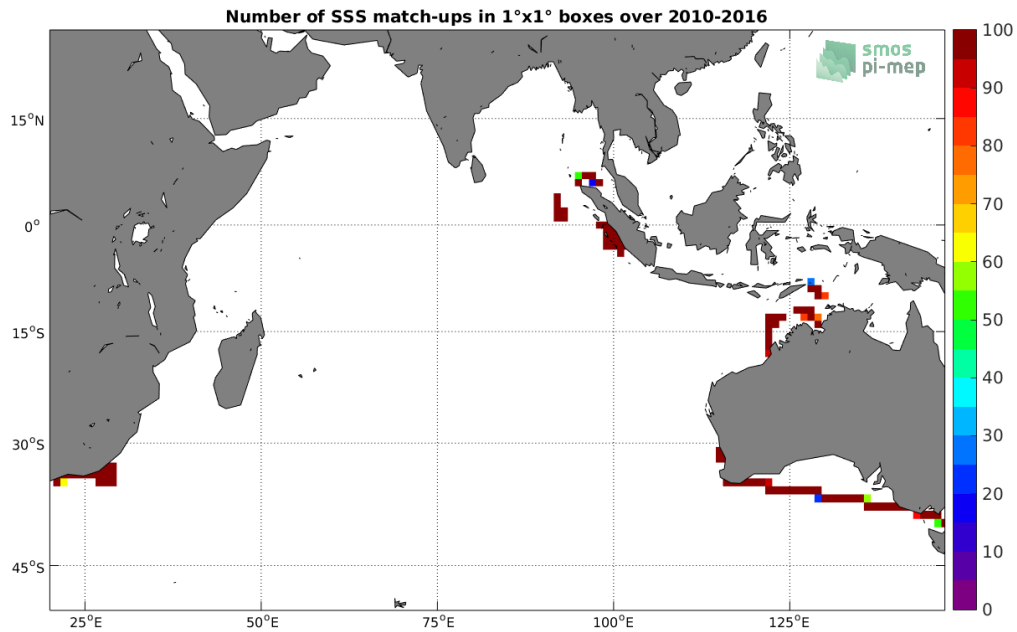
Figure 4: Number of SSS match-ups between TSG-SAMOS SSS and the SMOS-L3-CATDS-CECOS-LOCEAN-V3-18DAYS-25KM SSS product for the Indian Ocean Pi-MEP region over 1^\circ \times 1^\circ boxes and for the full satellite product period.
