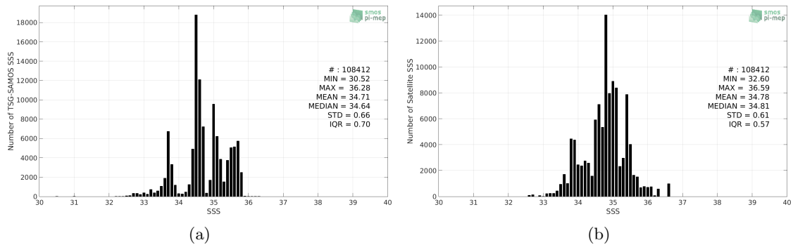
Figure 2: Histograms of SSS from TSG-SAMOS (a) and SMOS-L3-CATDS-CECOS-LOCEAN-V3-18DAYS-25KM (b) considering all match-up pairs per bins of 0.1 over the Indian Ocean Pi-MEP region and for the full satellite product period.
