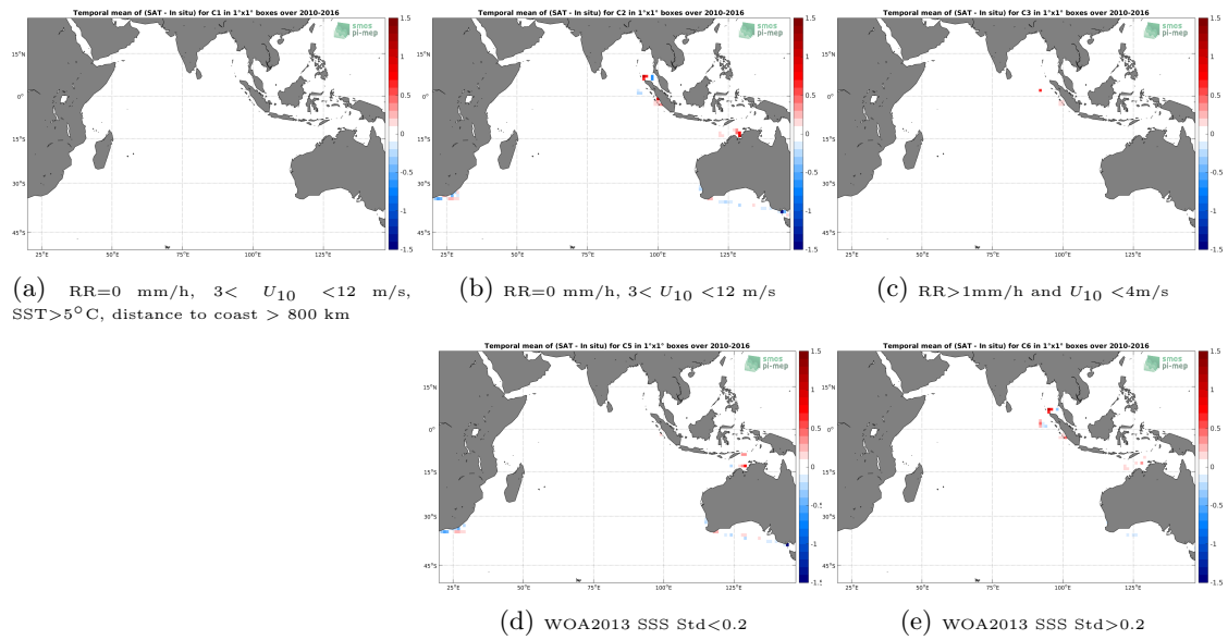
Figure 12: Temporal mean gridded over spatial boxes of size 1^\circ \times 1^\circ of \Delta SSS (SMOS-L3-CATDS-CECOS-LOCEAN-V3-18DAYS-25KM - TSG-SAMOS) for 5 different subdatasets corresponding to:RR=0 mm/h, 3 < U_{10} < 12 m/s, SST >5^\circ C, distance to coast > 800 km (a), RR=0 mm/h, 3 < U_{10} < 12 m/s (b), RR >1 mm/h and U_{10} < 4 m/s (c), WOA2013 SSS Std <0.2 (d), WOA2013 SSS Std >0.2 (e).
