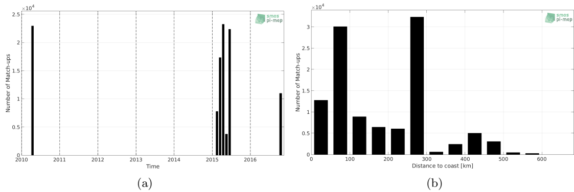
Figure 1: Number of match-ups between TSG-SAMOS and SMOS-L3-CATDS-CECOS-LOCEAN-V3-18DAYS-25KM SSS as a function of time (a) and as function of the distance to coast (b) over the Indian Ocean Pi-MEP region and for the full satellite product period.
