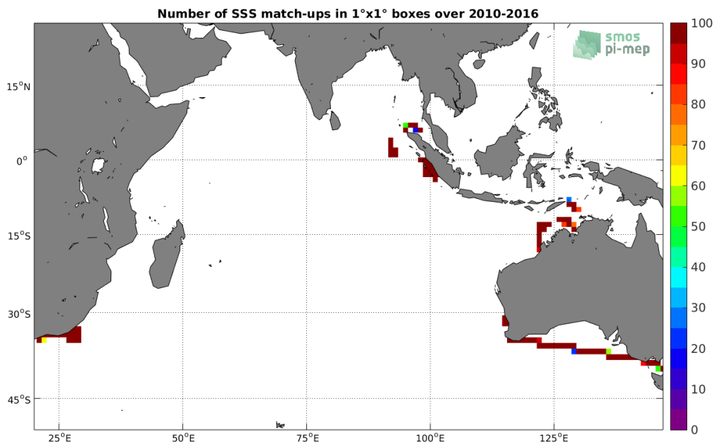
Figure 4: Number of SSS match-ups between TSG-SAMOS SSS and the SMOS-L3-CATDS-CECOS-LOCEAN-V3-18DAYS-25KM SSS product for the Indian Ocean Pi-MEP region over 1^\circ \times 1^\circ boxes and for the full satellite product period.
