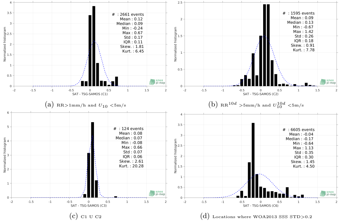
Figure 13: Normalized histogram of \Delta SSS (SMOS-L3-CATDS-CECOS-LOCEAN-V3-18DAYS-25KM - TSG-SAMOS) for 6 different subdatasets corresponding to: RR > 1mm/h and U_{10} < 5 m/s (a), RR^{10d} > 5 mm/h and U_{10}^{10d} < 5 m/s (b), C1 U C2 (c), Locations where WOA2013 SSS STD > 0.2 (d).
