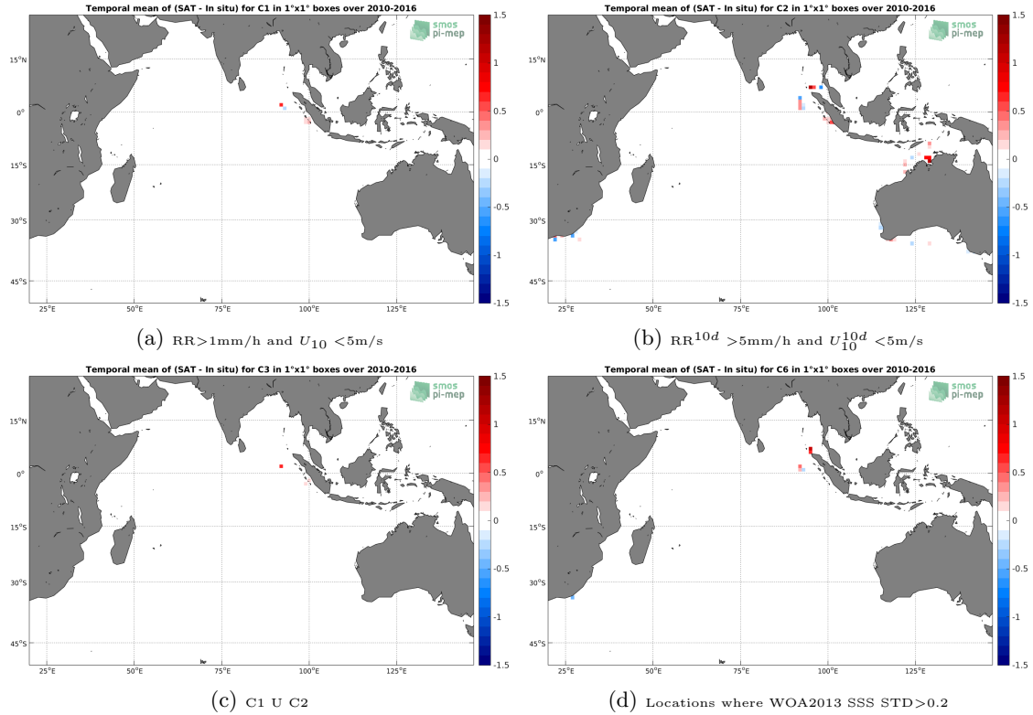
Figure 12: Temporal mean gridded over spatial boxes of size 1^\circ \times 1^\circ of \Delta SSS (SMOS-L3-CATDS-CECOS-LOCEAN-V3-18DAYS-25KM - TSG-SAMOS) for 4 different subdatasets corresponding to: RR > 1mm/h and U_{10} < 5 m/s (a), RR^{10d} > 5 mm/h and U_{10}^{10d} < 5 m/s (b), C1 U C2 (c), Locations where WOA2013 SSS STD > 0.2 (d).
