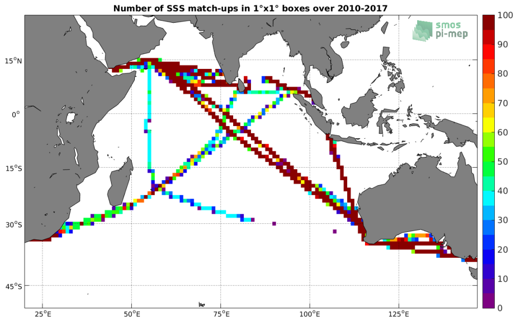
Figure 4: Number of SSS match-ups between TSG-LEGOS-DM SSS and the SMOS-L3-CATDS-CECOS-LOCEAN-V3-18DAYS-25KM SSS product for the Indian Ocean Pi-MEP region over 1°x1° boxes and for the full satellite product period.
