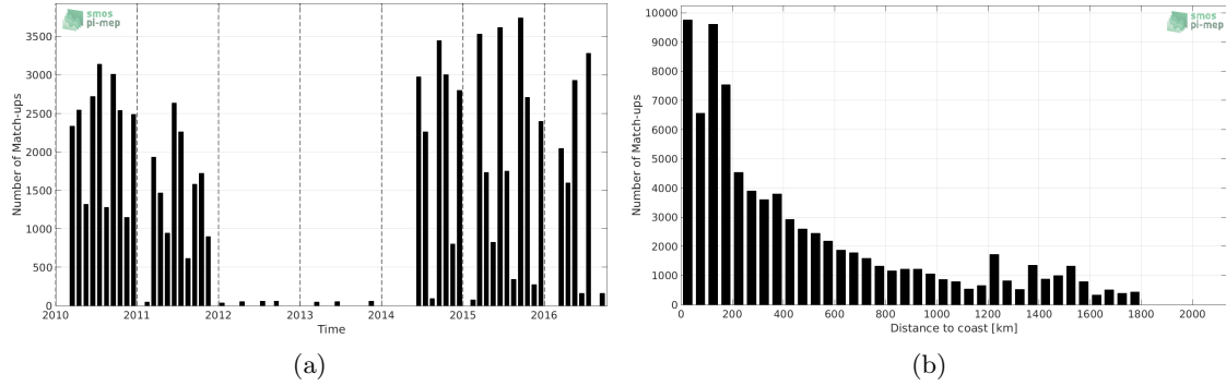
Figure 1: Number of match-ups between TSG-LEGOS-DM and SMOS-L3-CATDS-CECOS-LOCEAN-V3-18DAYS-25KM SSS as a function of time (a) and as function of the distance to coast (b) over the Indian Ocean Pi-MEP region and for the full satellite product period.
