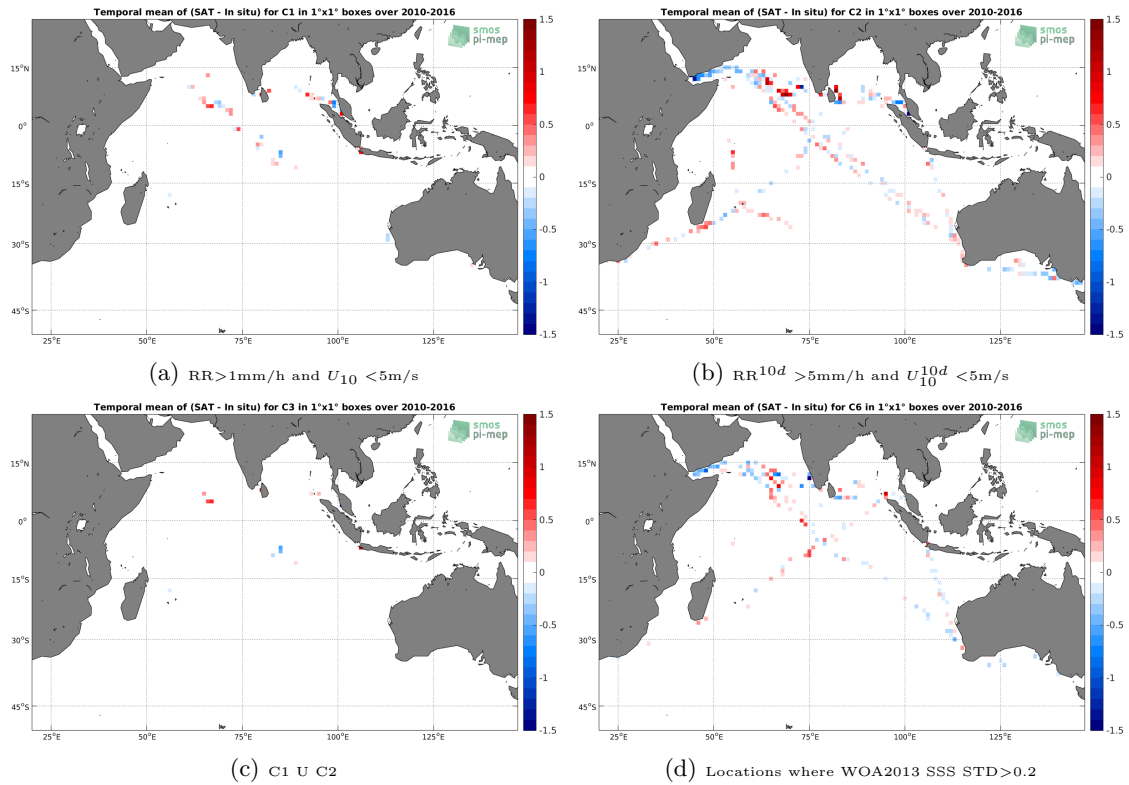
Figure 12: Temporal mean gridded over spatial boxes of size 1^\circ \times 1^\circ of \Delta SSS (SMOS-L3-CATDS-CECOS-LOCEAN-V3-18DAYS-25KM - TSG-LEGOS-DM) for 4 different subdatasets corresponding to: RR > 1\text{mm/h} and U_{10} < 5\text{m/s} (a), RR^{10d} > 5\text{mm/h} and U_{10}^{10d} < 5\text{m/s} (b), C1 U C2 (c), Locations where WOA2013 SSS STD > 0.2 (d).
