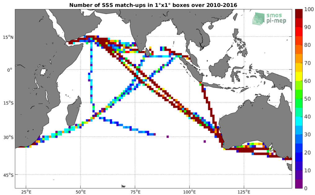
Figure 4: Number of SSS match-ups between TSG-LEGOS-DM SSS and the SMOS-L3-CATDS-CECOS-LOCEAN-V3-18DAYS-25KM SSS product for the Indian Ocean Pi-MEP region over 1^\circ \times 1^\circ boxes and for the full satellite product period.
