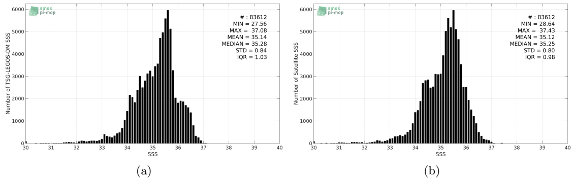
Figure 2: Histograms of SSS from TSG-LEGOS-DM (a) and SMOS-L3-CATDS-CECOS-LOCEAN-V3-18DAYS-25KM (b) considering all match-up pairs per bins of 0.1 over the Indian Ocean Pi-MEP region and for the full satellite product period.
