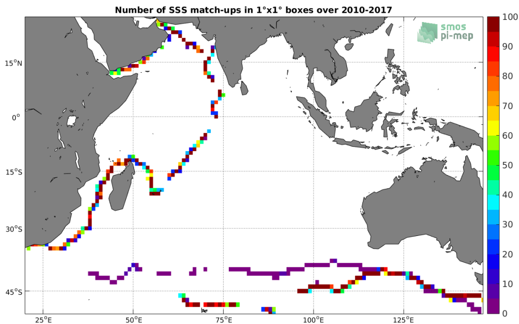
Figure 4: Number of SSS match-ups between TSG-GOSUD-Sailing-ship SSS and the SMOS-L3-CATDS-CECOS-LOCEAN-V3-18DAYS-25KM SSS product for the Indian Ocean Pi-MEP region over 1^\circ \times 1^\circ boxes and for the full satellite product period.
