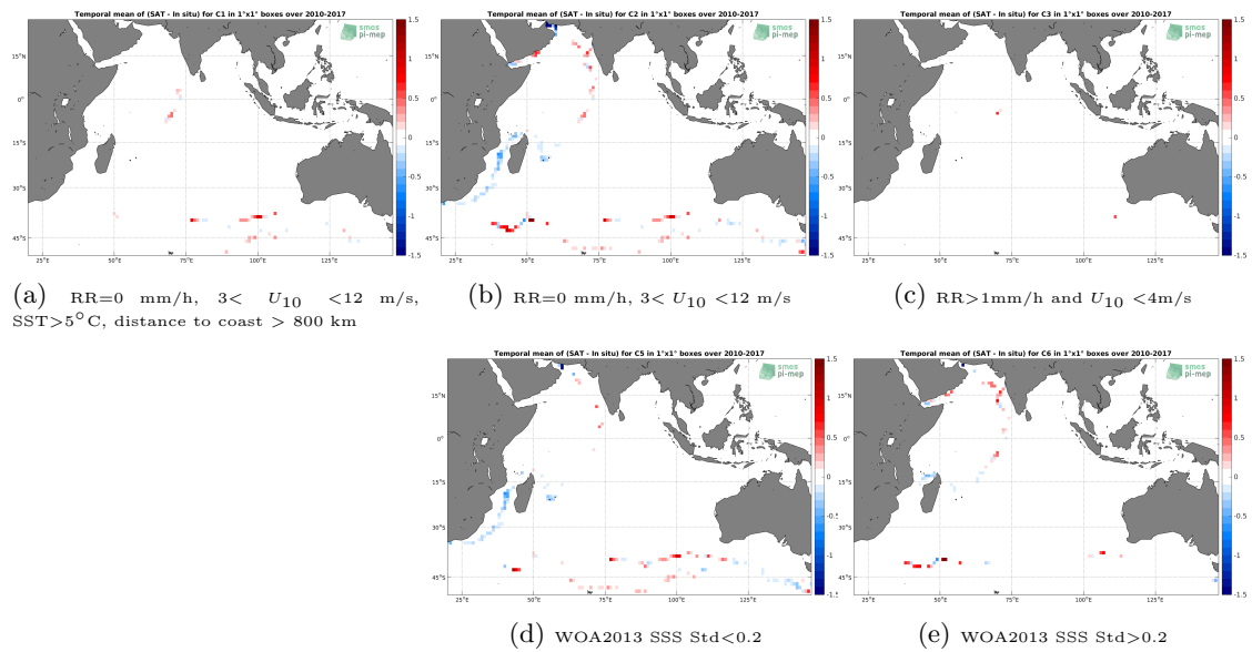
Figure 12: Temporal mean gridded over spatial boxes of size 1°x1° of \Delta SSS (SMOS-L3-CATDS-CECOS-LOCEAN-V3-18DAYS-25KM - TSG-GOSUD-Sailing-ship) for 5 different subdatasets corresponding to:RR=0 mm/h, 3 < U_{10} < 12 m/s, SST > 5°C, distance to coast > 800 km (a), RR=0 mm/h, 3 < U_{10} < 12 m/s (b), RR > 1mm/h and U_{10} < 4 m/s (c), WOA2013 SSS Std < 0.2 (d), WOA2013 SSS Std > 0.2 (e).
