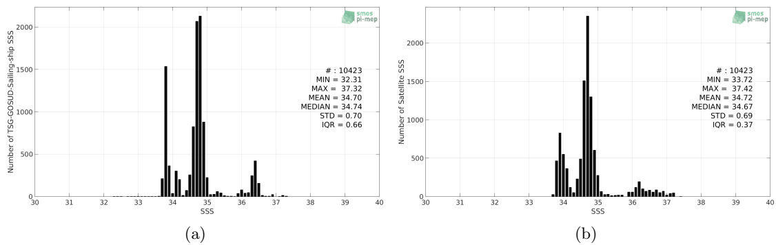
Figure 2: Histograms of SSS from TSG-GOSUD-Sailing-ship (a) and SMOS-L3-CATDS-CECOS-LOCEAN-V3-18DAYS-25KM (b) considering all match-up pairs per bins of 0.1 over the Indian Ocean Pi-MEP region and for the full satellite product period.
