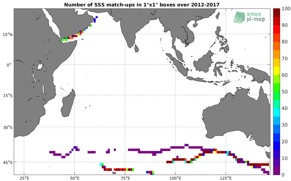
Figure 4: Number of SSS match-ups between TSG-GOSUD-Sailing-ship SSS and the SMOS-L3-CATDS-CECOS-LOCEAN-V3-18DAYS-25KM SSS product for the Indian Ocean Pi-MEP region over 1^\circ \times 1^\circ boxes and for the full satellite product period.
