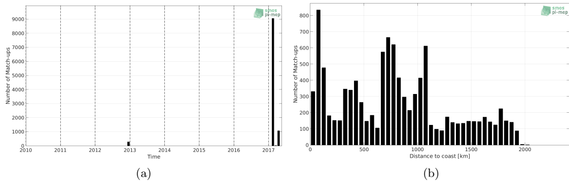
Figure 1: Number of match-ups between TSG-GOSUD-Sailing-ship and SMOS-L3-CATDS-CECOS-LOCEAN-V3-18DAYS-25KM SSS as a function of time (a) and as function of the distance to coast (b) over the Indian Ocean Pi-MEP region and for the full satellite product period.
