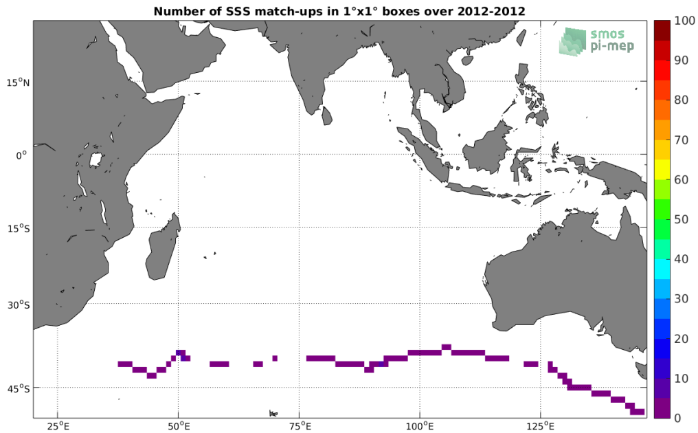
Figure 4: Number of SSS match-ups between TSG-GOSUD-Sailing-ship SSS and the SMOS-L3-CATDS-CECOS-LOCEAN-V3-18DAYS-25KM SSS product for the Indian Ocean Pi-MEP region over 1^{\circ} \times 1^{\circ} boxes and for the full satellite product period.
