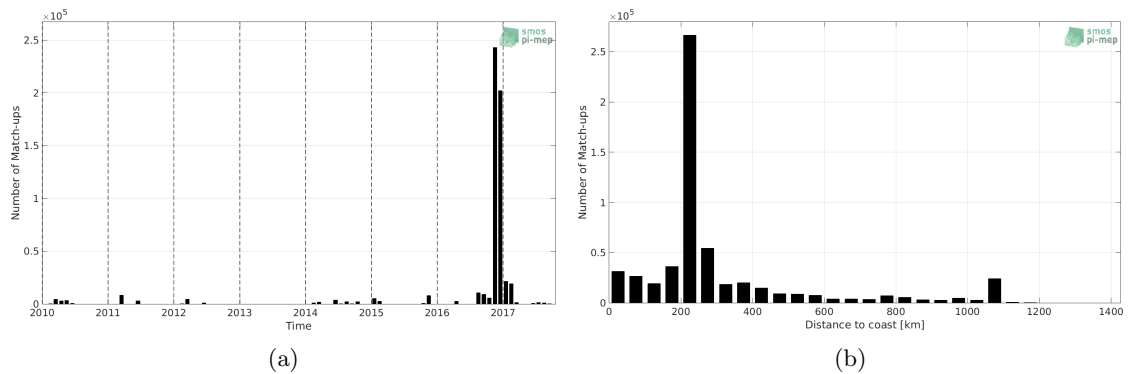
Figure 1: Number of match-ups between TSG-GOSUD-Research-vessel and SMOS-L3-CATDS-CECOS-LOCEAN-V3-18DAYS-25KM SSS as a function of time (a) and as function of distance to coast (b) over the Indian Ocean Pi-MEP region and for the full satellite product period.
