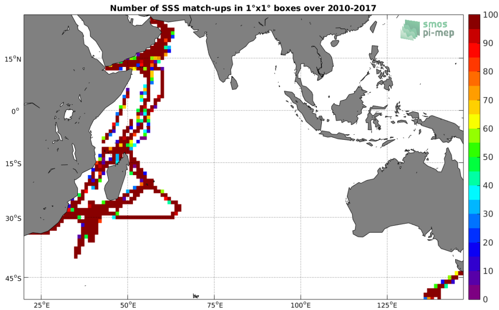
Figure 4: Number of SSS match-ups between TSG-GOSUD-Research-vessel SSS and the SMOS-L3-CATDS-CECOS-LOCEAN-V3-18DAYS-25KM SSS product for the Indian Ocean Pi-MEP region over 1^\circ \times 1^\circ boxes and for the full satellite product period.
