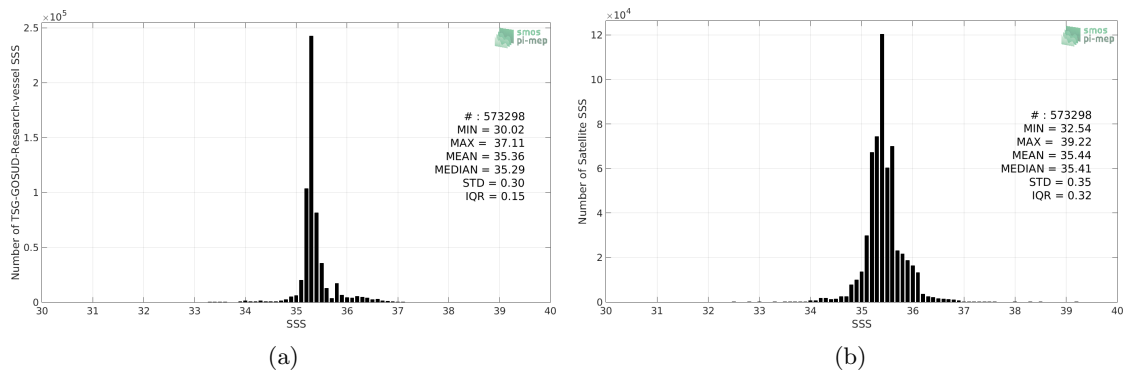
Figure 2: Histograms of SSS from TSG-GOSUD-Research-vessel (a) and SMOS-L3-CATDS-CECOS-LOCEAN-V3-18DAYS-25KM (b) considering all match-up pairs per bins of 0.1 over the Indian Ocean Pi-MEP region and for the full satellite product period.
