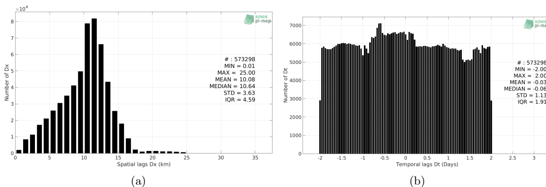
Figure 5: Histograms of the spatial (a) and temporal (b) lags between the time of the TSG-GOSUD-Research-vessel measurements and the date of the corresponding SMOS-L3-CATDS-CECOS-LOCEAN-V3-18DAYS-25KM SSS product.
