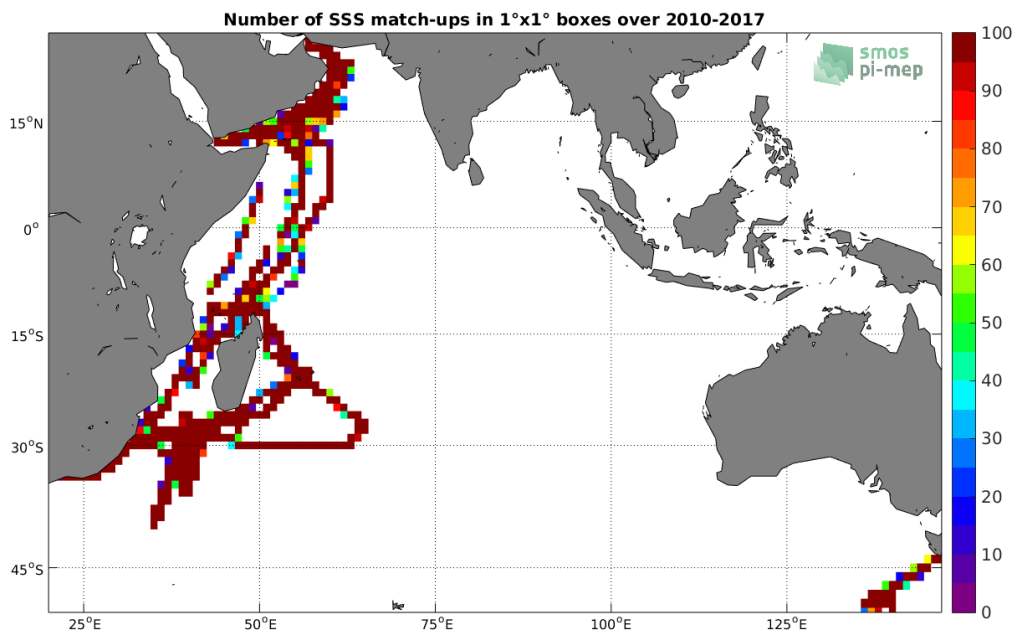
Figure 4: Number of SSS match-ups between TSG-GOSUD-Research-vessel SSS and the SMOS-L3-CATDS-CECOS-LOCEAN-V3-18DAYS-25KM SSS product for the Indian Ocean Pi-MEP region over 1°x1° boxes and for the full satellite product period.
