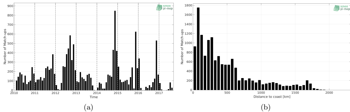
Figure 1: Number of match-ups between Sea mammals and SMOS-L3-CATDS-CECOS-LOCEAN-V3-18DAYS-25KM SSS as a function of time (a) and as function of the distance to coast (b) over the Indian Ocean Pi-MEP region and for the full satellite product period.
