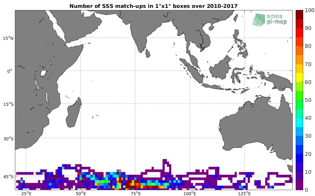
Figure 4: Number of SSS match-ups between Sea mammals SSS and the SMOS-L3-CATDS-CECOS-LOCEAN-V3-18DAYS-25KM SSS product for the Indian Ocean Pi-MEP region over 1°x1° boxes and for the full satellite product period.
