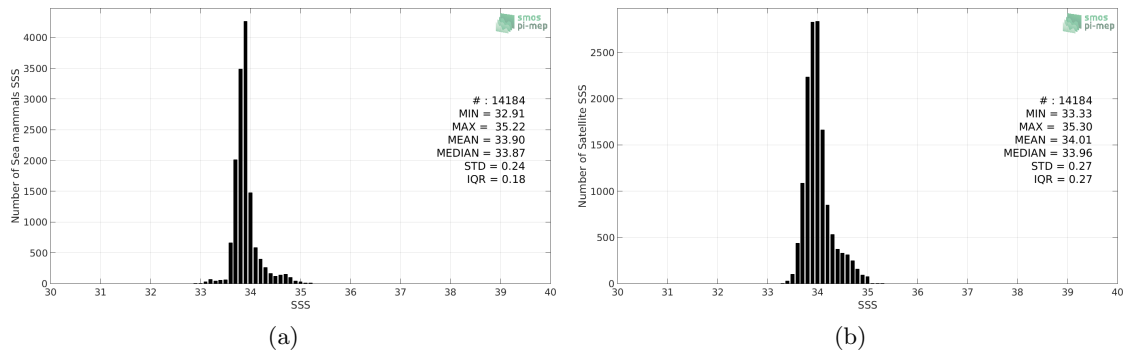
Figure 2: Histograms of SSS from Sea mammals (a) and SMOS-L3-CATDS-CECOS-LOCEAN-V3-18DAYS-25KM (b) considering all match-up pairs per bins of 0.1 over the Indian Ocean Pi-MEP region and for the full satellite product period.
