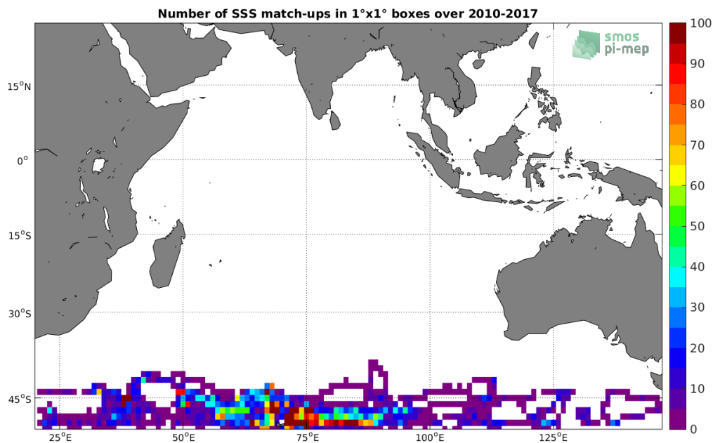
Figure 4: Number of SSS match-ups between Sea mammals SSS and the SMOS-L3-CATDS-CECOS-LOCEAN-V3-18DAYS-25KM SSS product for the Indian Ocean Pi-MEP region over 1^{\circ} \times 1^{\circ} boxes and for the full satellite product period.
