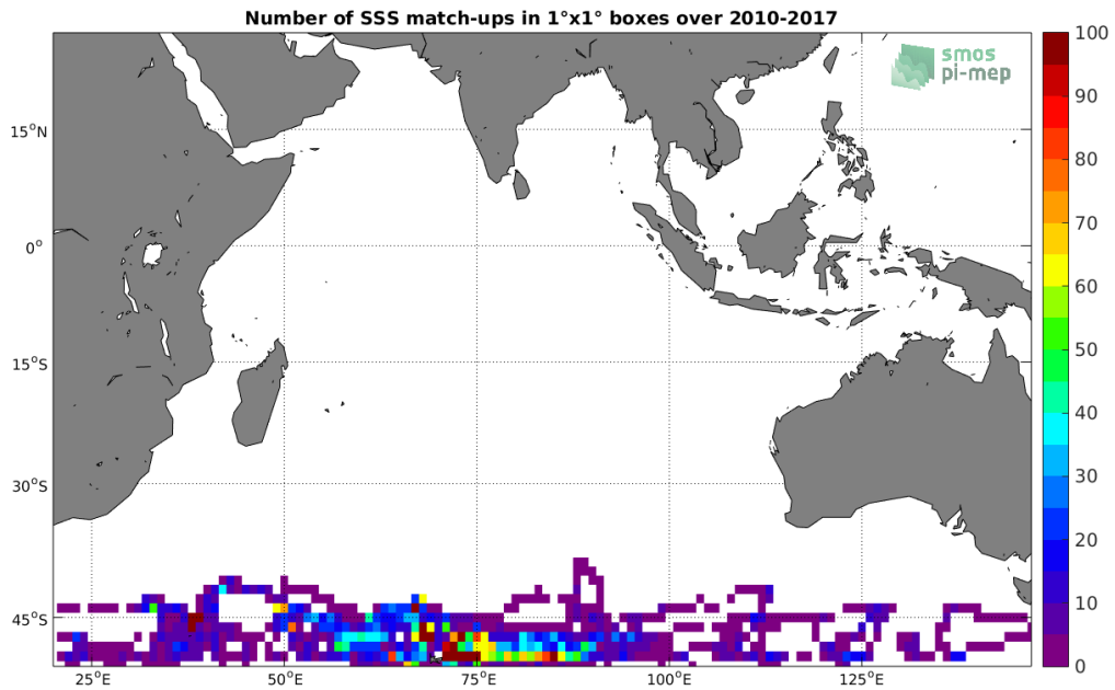
Figure 4: Number of SSS match-ups between Sea mammals SSS and the SMOS-L3-CATDS-CECOS-LOCEAN-V3-18DAYS-25KM SSS product for the Indian Ocean Pi-MEP region over 1^\circ \times 1^\circ boxes and for the full satellite product period.
