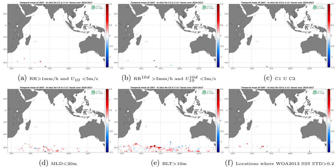
Figure 12: Temporal mean gridded over spatial boxes of size 1^\circ \times 1^\circ of \Delta\text{SSS} (SMOS-L3-CATDS-CECOS-LOCEAN-V3-18DAYS-25KM - Sea mammals) for 6 different subdatasets corresponding to: RR > 1\text{mm/h} and U_{10} < 5\text{m/s} (a), RR^{10d} > 5\text{mm/h} and U_{10}^{10d} < 5\text{m/s} (b), C1 U C2 (c), MLD < 20\text{m} (d), BLT > 10\text{m} (e), Locations where WOA2013 SSS STD > 0.2 (f).
