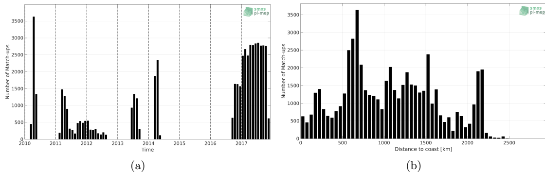
Figure 1: Number of match-ups between Surface drifters and SMOS-L3-CATDS-CECOS-LOCEAN-V3-18DAYS-25KM SSS as a function of time (a) and as function of the distance to coast (b) over the Indian Ocean Pi-MEP region and for the full satellite product period.
