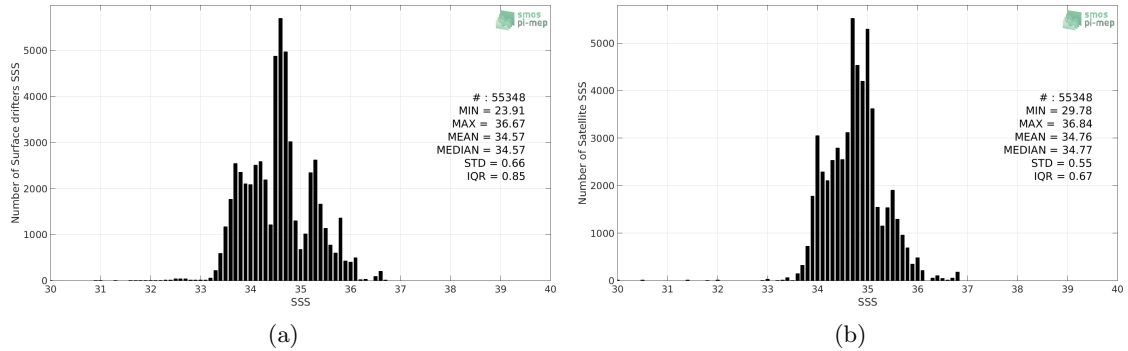
Figure 2: Histograms of SSS from Surface drifters (a) and SMOS-L3-CATDS-CECOS-LOCEAN-V3-18DAYS-25KM (b) considering all match-up pairs per bins of 0.1 over the Indian Ocean Pi-MEP region and for the full satellite product period.
