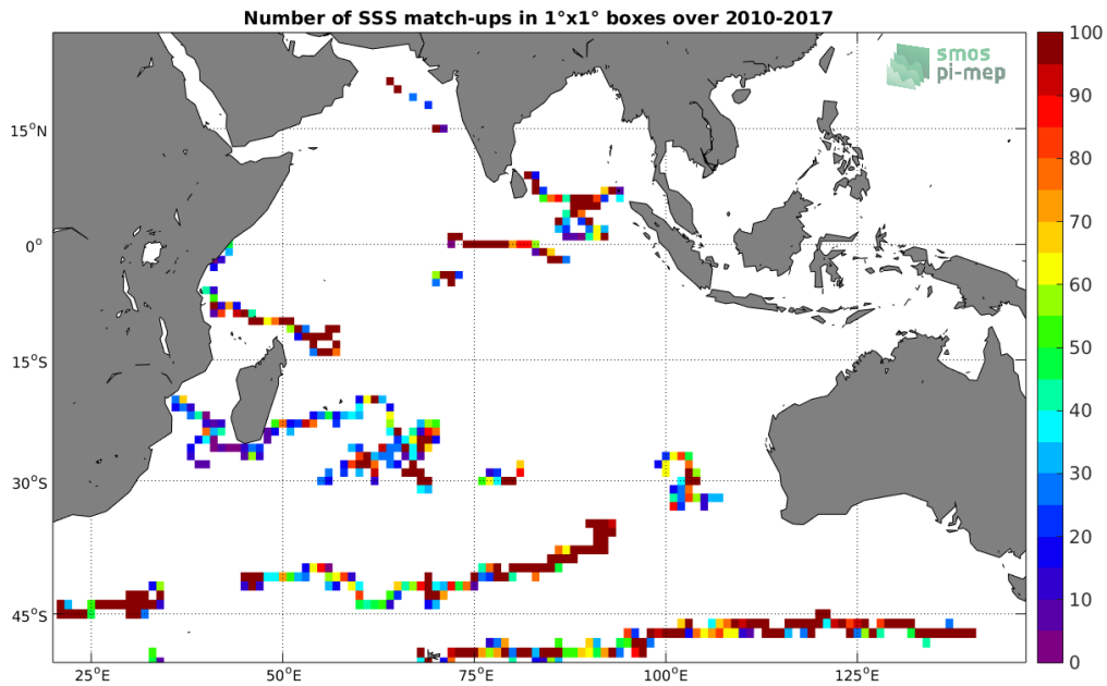
Figure 3: Number of SSS match-ups between Surface drifters SSS and the SMOS-L3-CATDS-CECOS-LOCEAN-V3-18DAYS-25KM SSS product for the Indian Ocean Pi-MEP region over 1^\circ \times 1^\circ boxes and for the full satellite product period.
