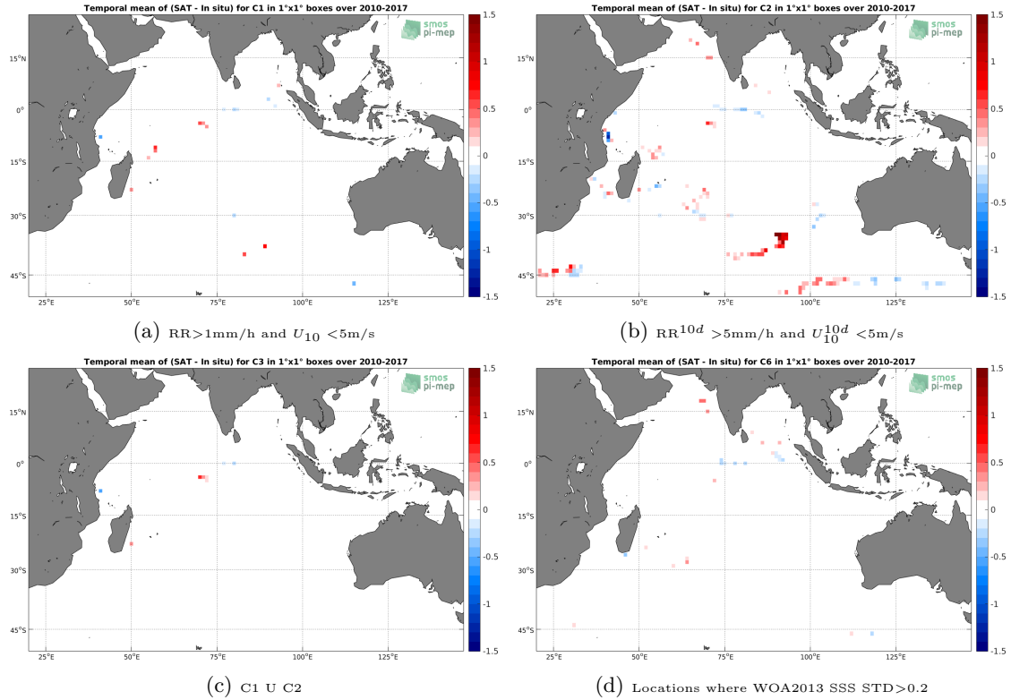
Figure 11: Temporal mean gridded over spatial boxes of size 1^\circ \times 1^\circ of \Delta SSS (SMOS-L3-CATDS-CECOS-LOCEAN-V3-18DAYS-25KM - Surface drifters) for 4 different subdatasets corresponding to: RR > 1\text{mm/h} and U_{10} < 5\text{m/s} (a), RR^{10d} > 5\text{mm/h} and U_{10}^{10d} < 5\text{m/s} (b), C1 U C2 (c), Locations where WOA2013 SSS STD > 0.2 (d).
