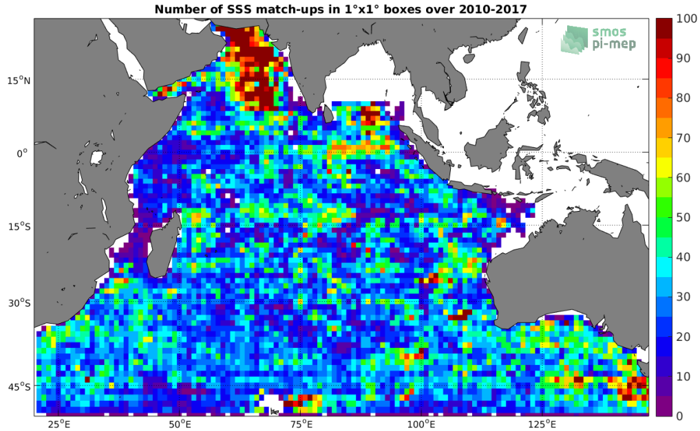
Figure 4: Number of SSS match-ups between Argos SSS and the SMOS-L3-CATDS-CECOS-LOCEAN-V3-18DAYS-25KM SSS product for the Indian Ocean Pi-MEP region over 1°x1° boxes and for the full satellite product period.
