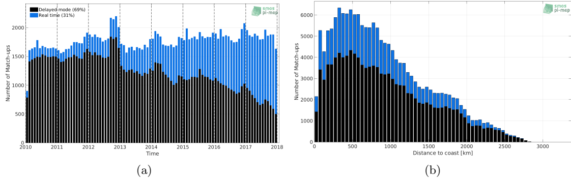
Figure 1: Number of match-ups between Argo and SMOS-L3-CATDS-CECOS-LOCEAN-V3-18DAYS-25KM SSS as a function of time (a) and as function of the distance to coast (b) over the Indian Ocean Pi-MEP region and for the full satellite product period.
