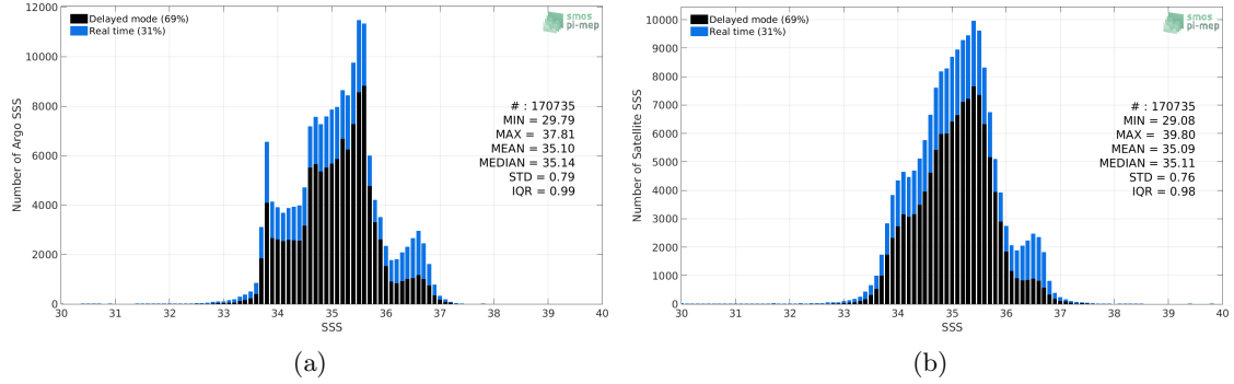
Figure 2: Histograms of SSS from Argo (a) and SMOS-L3-CATDS-CECOS-LOCEAN-V3-18DAYS-25KM (b) considering all match-up pairs per bins of 0.1 over the Indian Ocean Pi-MEP region and for the full satellite product period.
