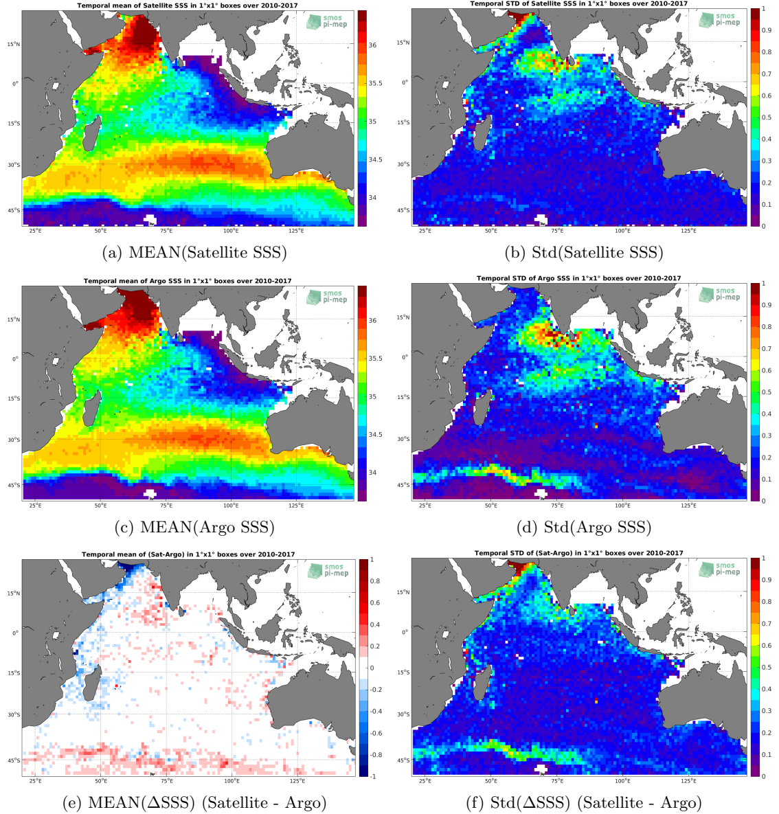
Figure 6: Temporal mean (left) and Std (right) of SSS from SMOS-L3-CATDS-CECOS-LOCEAN-V3-18DAYS-25KM (top), Argo (middle), and of \Delta SSS (Satellite - Argo). Only match-up pairs are used to generate these maps.
