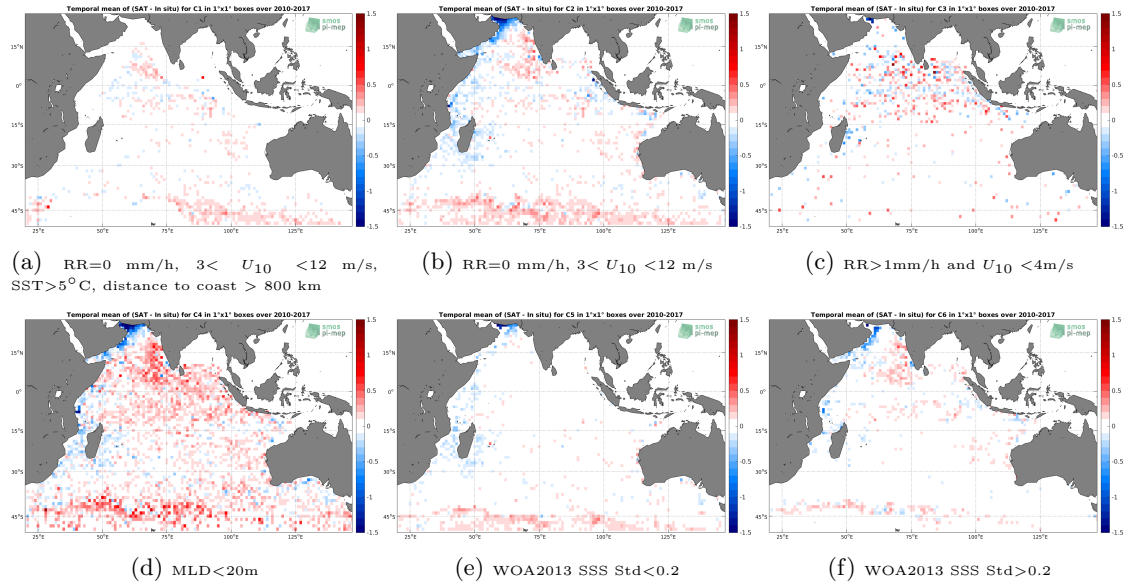
Figure 12: Temporal mean gridded over spatial boxes of size 1^\circ \times 1^\circ of \Delta SSS (SMOS-L3-CATDS-CECOS-LOCEAN-V3-18DAYS-25KM - Argo) for 6 different subdatasets corresponding to: RR=0 mm/h, 3 < U_{10} < 12 m/s, SST > 5^\circ C , distance to coast > 800 km (a), RR=0 mm/h, 3 < U_{10} < 12 m/s (b), RR > 1 mm/h and U_{10} < 4 m/s (c), MLD < 20 m (d), WOA2013 SSS Std < 0.2 (e), WOA2013 SSS Std > 0.2 (f).
