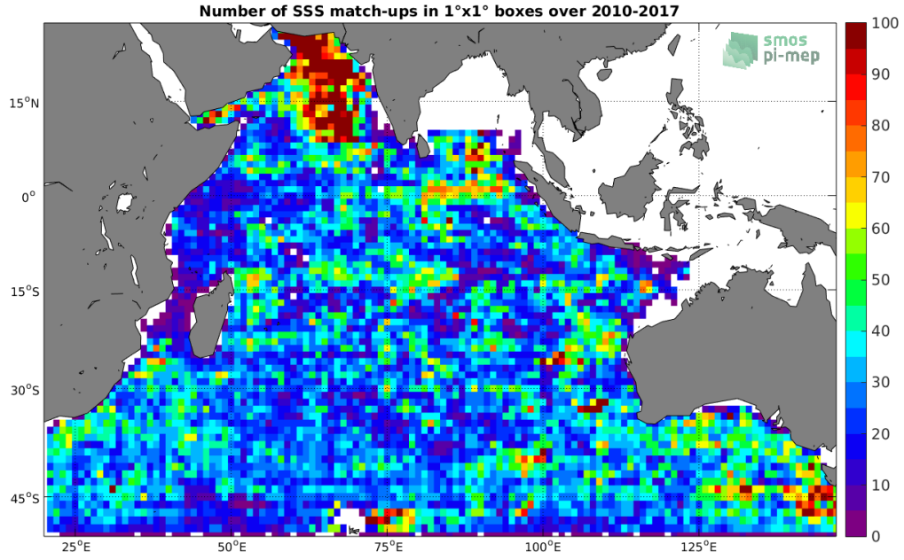
Figure 4: Number of SSS match-ups between Argo SSS and the SMOS-L3-CATDS-CECOS-LOCEAN-V3-18DAYS-25KM SSS product for the Indian Ocean Pi-MEP region over 1^\circ \times 1^\circ boxes and for the full satellite product period.
