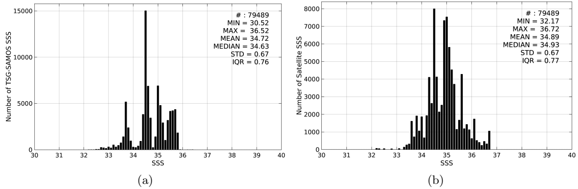
Figure 2: Histograms of SSS from TSG-SAMOS (a) and SMOS-L3-CATDS-CECOS-LOCEAN-V2-9DAYS-25KM (b) considering all match-up pairs per bins of 0.1 over the Indian Ocean Pi-MEP region and for the full satellite product period.
