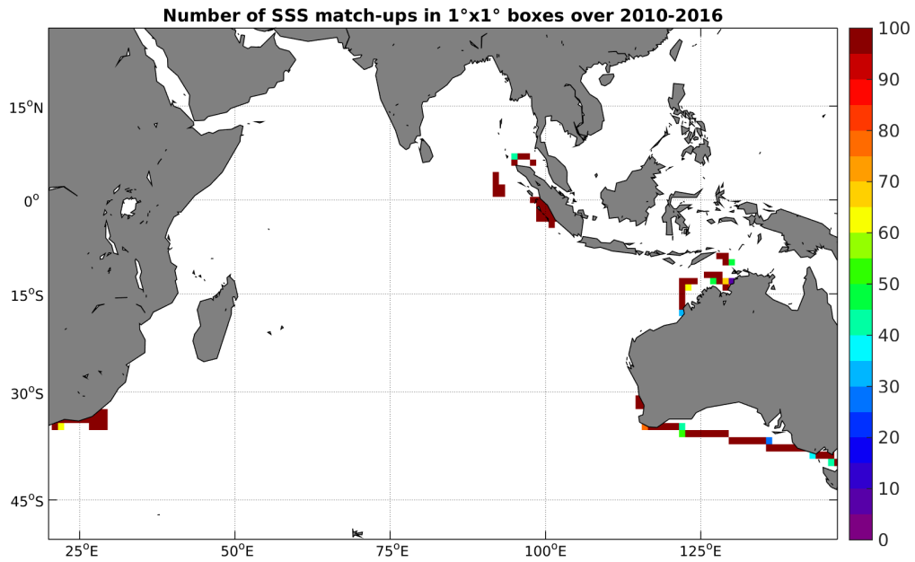
Figure 4: Number of SSS match-ups between TSG-SAMOS SSS and the SMOS-L3-CATDS-CECOS-LOCEAN-V2-9DAYS-25KM SSS product for the Indian Ocean Pi-MEP region over 1^\circ \times 1^\circ boxes and for the full satellite product period.
