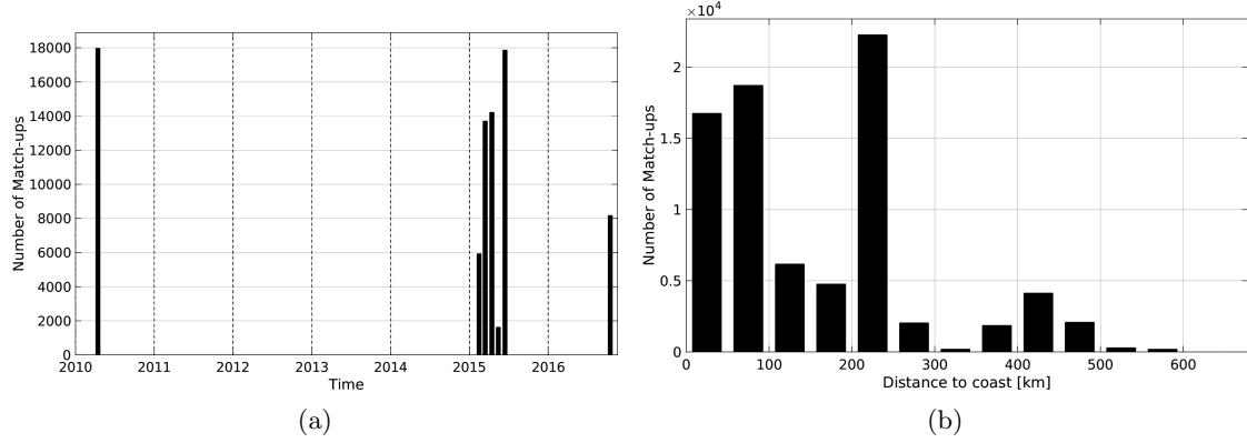
Figure 1: Number of match-ups between TSG-SAMOS and SMOS-L3-CATDS-CECOS-LOCEAN-V2-9DAYS-25KM SSS as a function of time (a) and as function of the distance to coast (b) over the Indian Ocean Pi-MEP region and for the full satellite product period.
