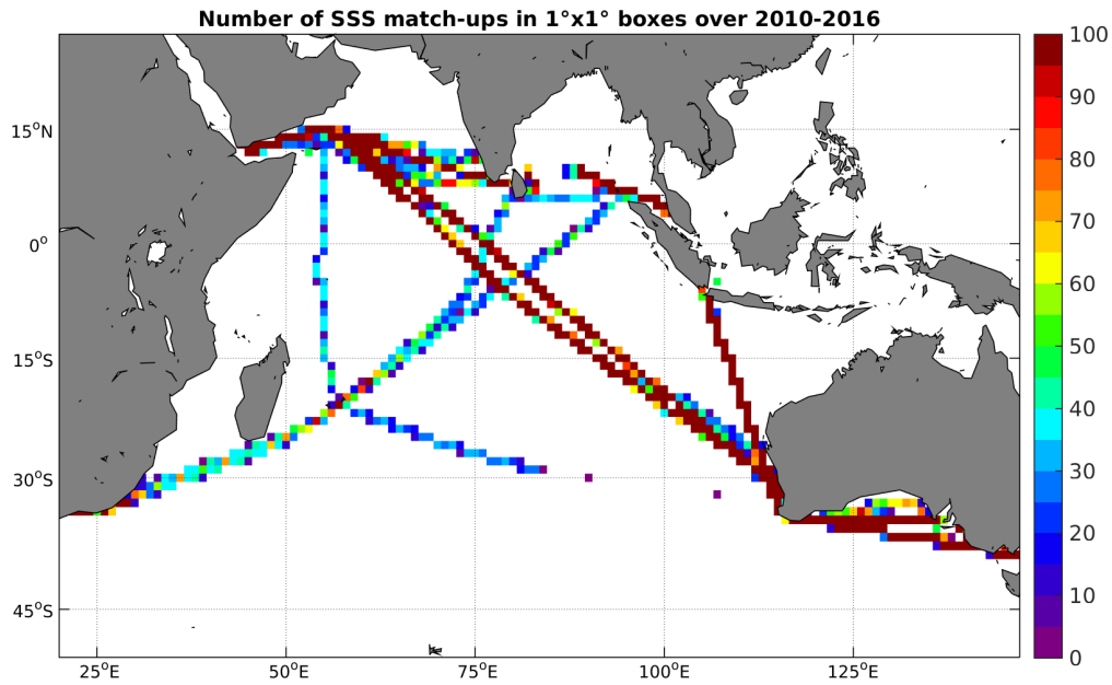
Figure 4: Number of SSS match-ups between TSG-LEGOS-DM SSS and the SMOS-L3-CATDS-CECOS-LOCEAN-V2-9DAYS-25KM SSS product for the Indian Ocean Pi-MEP region over 1°x1° boxes and for the full satellite product period.
