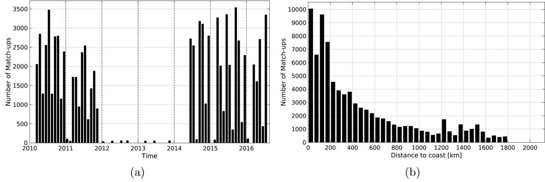
Figure 1: Number of match-ups between TSG-LEGOS-DM and SMOS-L3-CATDS-CECOS-LOCEAN-V2-9DAYS-25KM SSS as a function of time (a) and as function of the distance to coast (b) over the Indian Ocean Pi-MEP region and for the full satellite product period.
