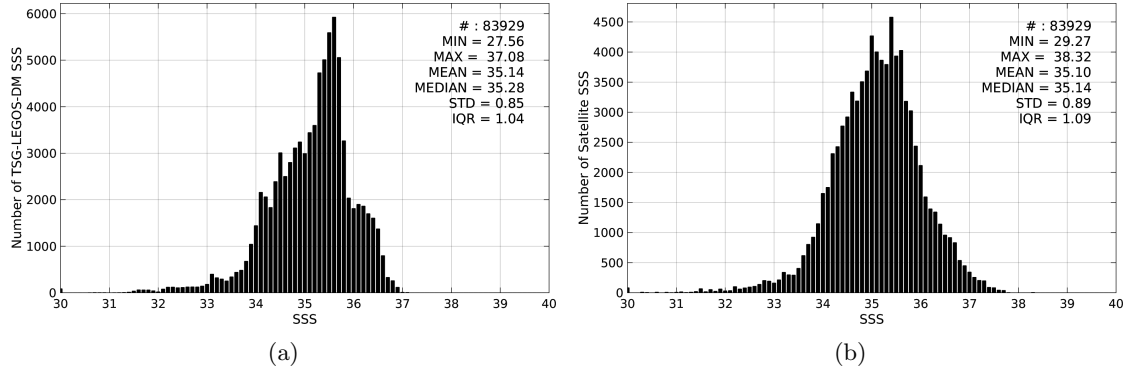
Figure 2: Histograms of SSS from TSG-LEGOS-DM (a) and SMOS-L3-CATDS-CECOS-LOCEAN-V2-9DAYS-25KM (b) considering all match-up pairs per bins of 0.1 over the Indian Ocean Pi-MEP region and for the full satellite product period.
