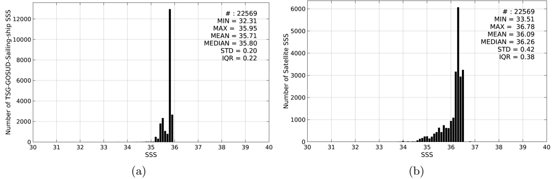
Figure 2: Histograms of SSS from TSG-GOSUD-Sailing-ship (a) and SMOS-L3-CATDS-CECOS-LOCEAN-V2-9DAYS-25KM (b) considering all match-up pairs per bins of 0.1 over the Indian Ocean Pi-MEP region and for the full satellite product period.
