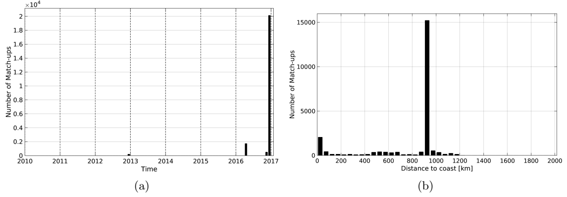
Figure 1: Number of match-ups between TSG-GOSUD-Sailing-ship and SMOS-L3-CATDS-CECOS-LOCEAN-V2-9DAYS-25KM SSS as a function of time (a) and as function of the distance to coast (b) over the Indian Ocean Pi-MEP region and for the full satellite product period.
