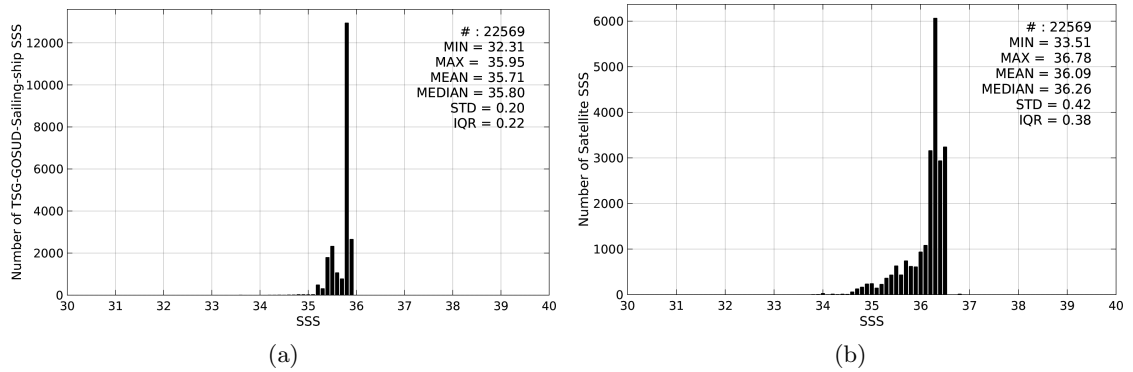
Figure 2: Histograms of SSS from TSG-GOSUD-Sailing-ship (a) and SMOS-L3-CATDS-CECOS-LOCEAN-V2-9DAYS-25KM (b) considering all match-up pairs per bins of 0.1 over the Indian Ocean Pi-MEP region and for the full satellite product period.
