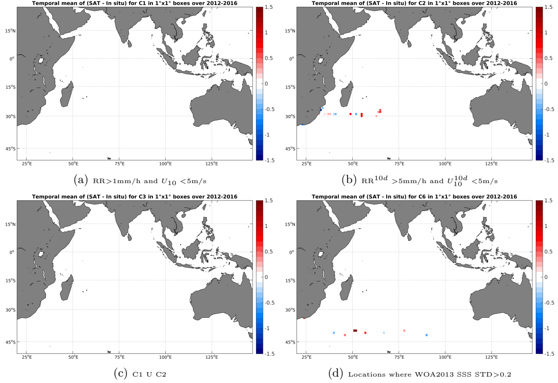
Figure 12: Temporal mean gridded over spatial boxes of size 1^\circ \times 1^\circ of \Delta SSS (SMOS-L3-CATDS-CECOS-LOCEAN-V2-9DAYS-25KM - TSG-GOSUD-Sailing-ship) for 4 different subdatasets corresponding to: RR > 1\text{mm/h} and U_{10} < 5\text{m/s} (a), RR^{10d} > 5\text{mm/h} and U_{10}^{10d} < 5\text{m/s} (b), C1 U C2 (c), Locations where WOA2013 SSS STD > 0.2 (d).
