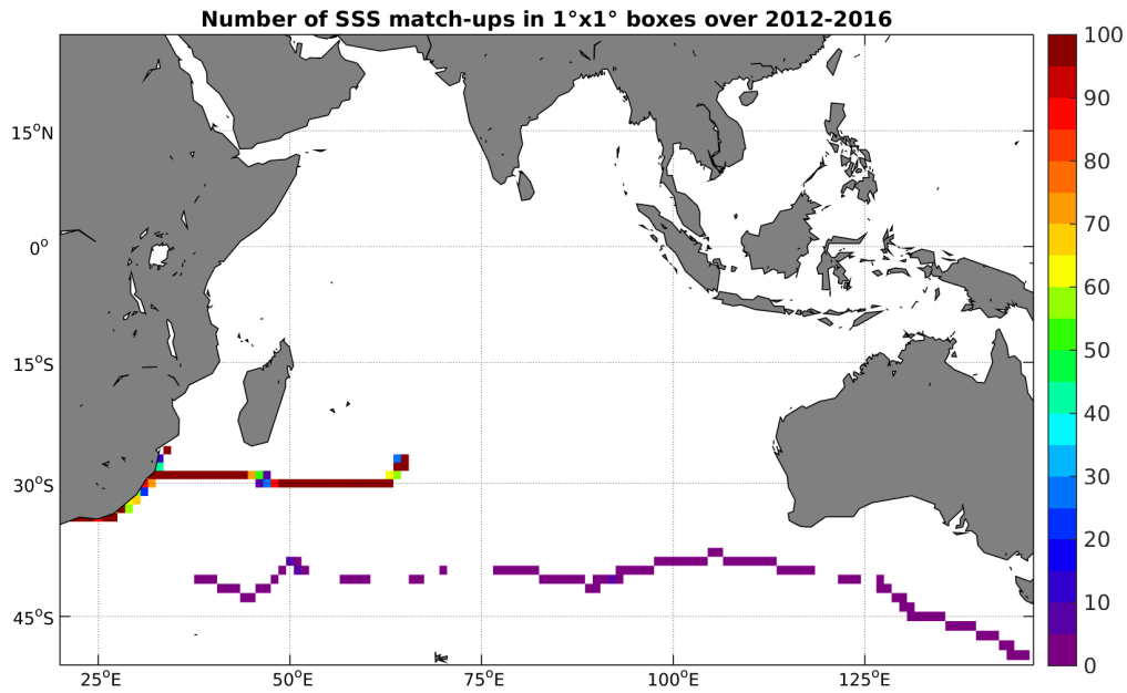
Figure 4: Number of SSS match-ups between TSG-GOSUD-Sailing-ship SSS and the SMOS-L3-CATDS-CECOS-LOCEAN-V2-9DAYS-25KM SSS product for the Indian Ocean Pi-MEP region over 1°x1° boxes and for the full satellite product period.
