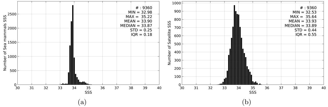
Figure 2: Histograms of SSS from Sea mammals (a) and SMOS-L3-CATDS-CECOS-LOCEAN-V2-9DAYS-25KM (b) considering all match-up pairs per bins of 0.1 over the Indian Ocean Pi-MEP region and for the full satellite product period.
