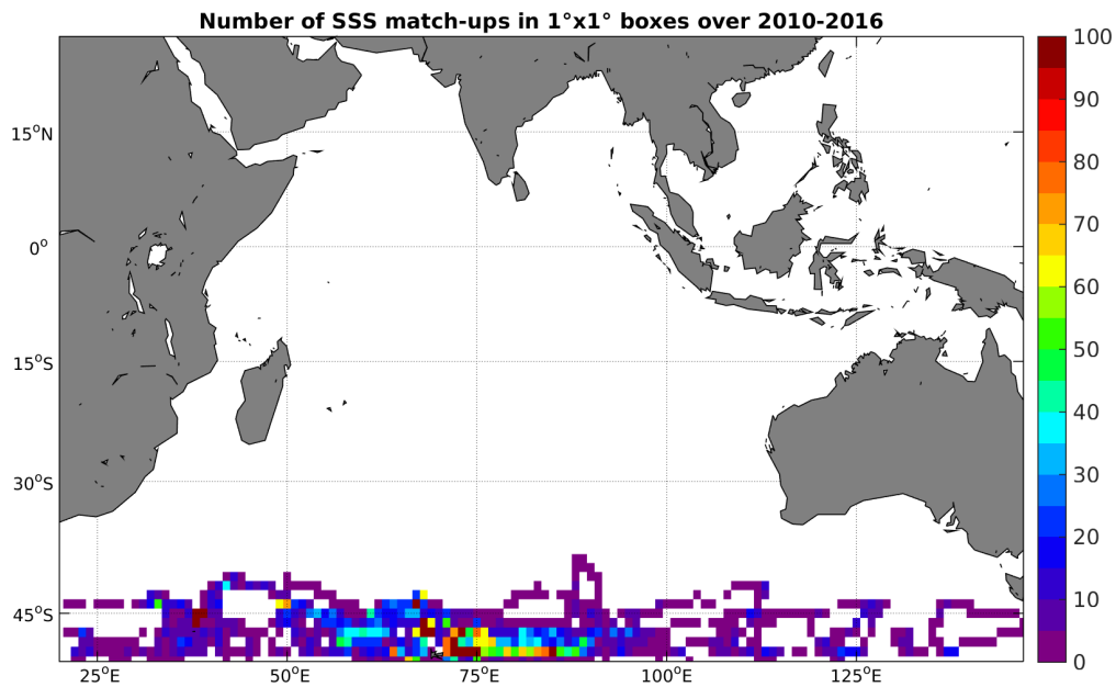
Figure 4: Number of SSS match-ups between Sea mammals SSS and the SMOS-L3-CATDS-CECOS-LOCEAN-V2-9DAYS-25KM SSS product for the Indian Ocean Pi-MEP region over 1^\circ \times 1^\circ boxes and for the full satellite product period.
