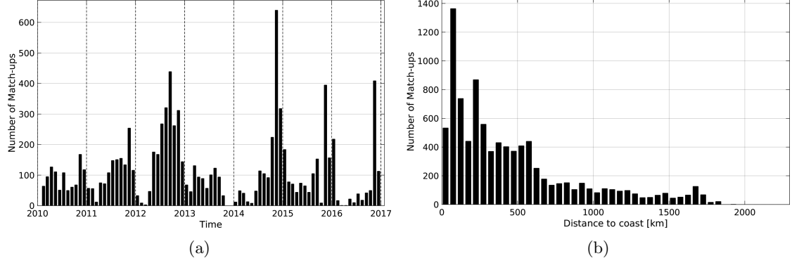
Figure 1: Number of match-ups between Sea mammals and SMOS-L3-CATDS-CECOS-LOCEAN-V2-9DAYS-25KM SSS as a function of time (a) and as function of the distance to coast (b) over the Indian Ocean Pi-MEP region and for the full satellite product period.
