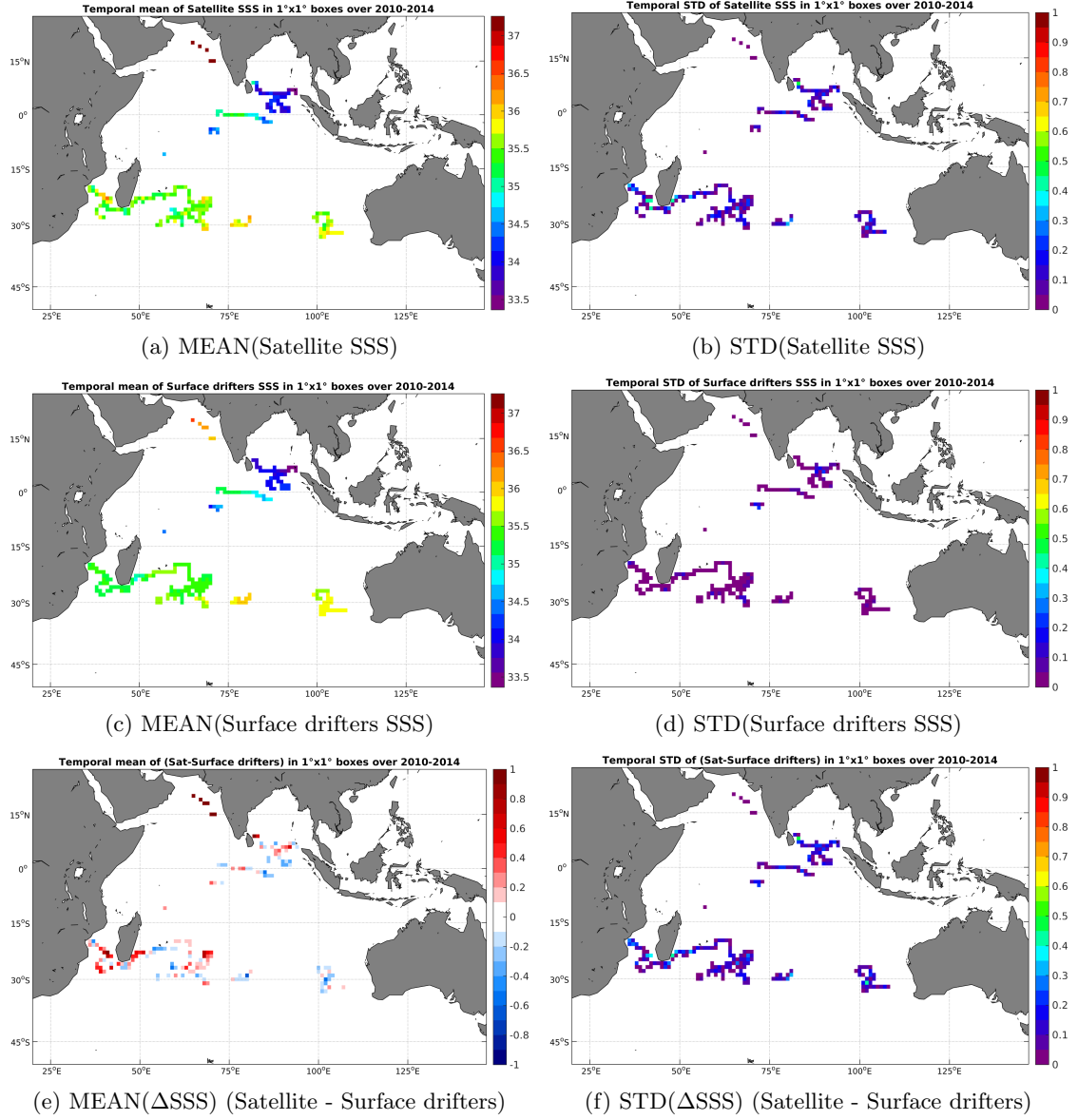
Figure 5: Temporal mean (left) and STD (right) of SSS from SMOS-L3-CATDS-CECOS-LOCEAN-V2-9DAYS-25KM (top), Surface drifters (middle), and of \Delta SSS (Satellite - Surface drifters). Only match-up pairs are used to generate these maps.
