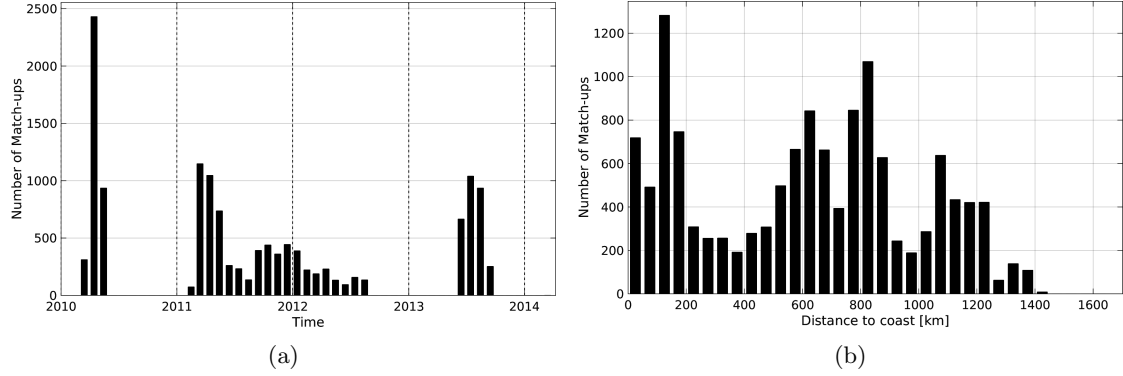
Figure 1: Number of match-ups between Surface drifters and SMOS-L3-CATDS-CECOS-LOCEAN-V2-9DAYS-25KM SSS as a function of time (a) and as function of the distance to coast (b) over the Indian Ocean Pi-MEP region and for the full satellite product period.
