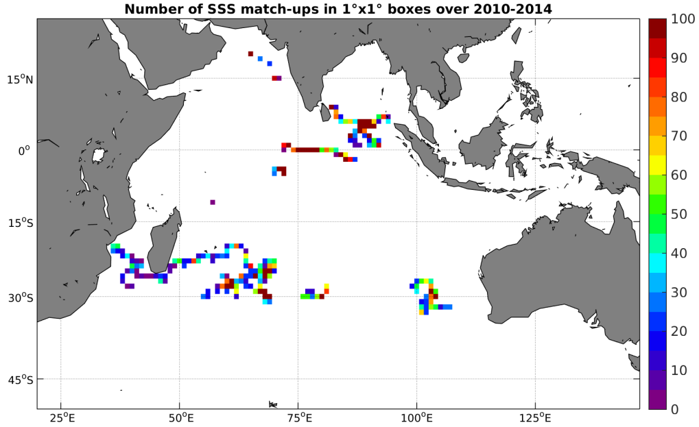
Figure 3: Number of SSS match-ups between Surface drifters SSS and the SMOS-L3-CATDS-CECOS-LOCEAN-V2-9DAYS-25KM SSS product for the Indian Ocean Pi-MEP region over 1^\circ \times 1^\circ boxes and for the full satellite product period.
