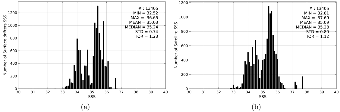
Figure 2: Histograms of SSS from Surface drifters (a) and SMOS-L3-CATDS-CECOS-LOCEAN-V2-9DAYS-25KM (b) considering all match-up pairs per bins of 0.1 over the Indian Ocean Pi-MEP region and for the full satellite product period.
