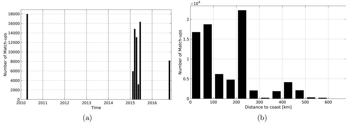
Figure 1: Number of match-ups between TSG-SAMOS and SMOS-L3-CATDS-CECOS-LOCEAN-V2-18DAYS-25KM SSS as a function of time (a) and as function of the distance to coast (b) over the Indian Ocean Pi-MEP region and for the full satellite product period.
