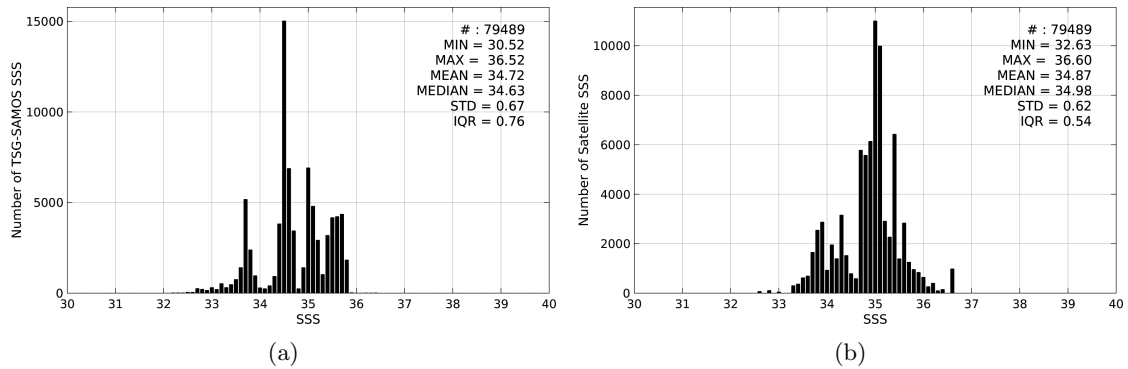
Figure 2: Histograms of SSS from TSG-SAMOS (a) and SMOS-L3-CATDS-CECOS-LOCEAN-V2-18DAYS-25KM (b) considering all match-up pairs per bins of 0.1 over the Indian Ocean Pi-MEP region and for the full satellite product period.
