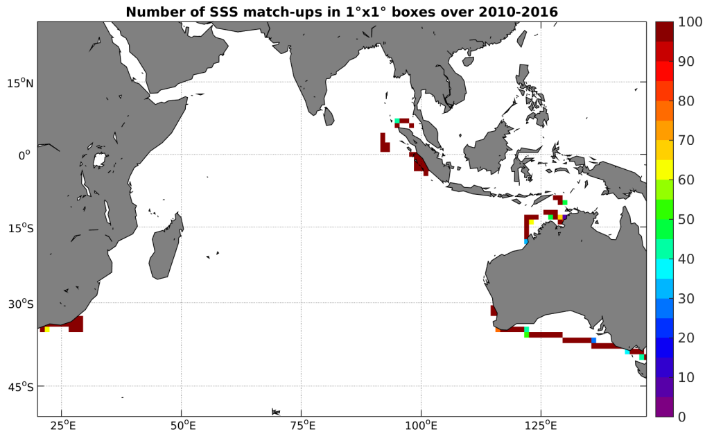
Figure 4: Number of SSS match-ups between TSG-SAMOS SSS and the SMOS-L3-CATDS-CECOS-LOCEAN-V2-18DAYS-25KM SSS product for the Indian Ocean Pi-MEP region over 1^\circ \times 1^\circ boxes and for the full satellite product period.
