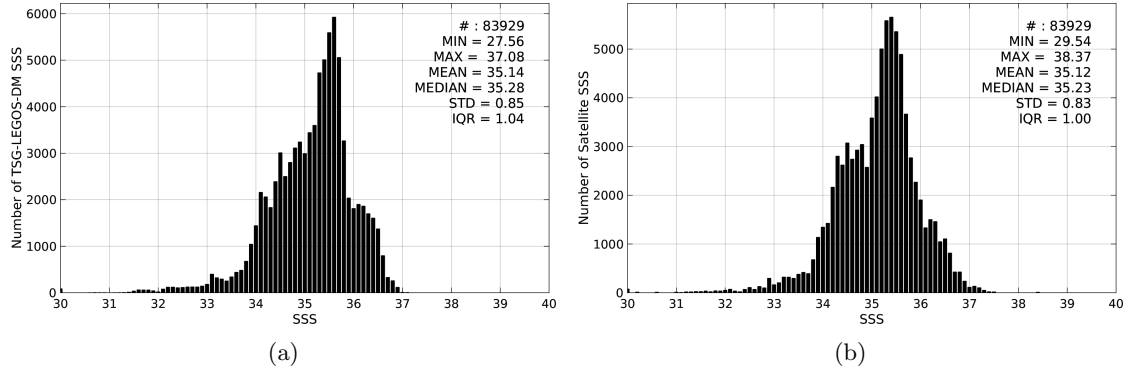
Figure 2: Histograms of SSS from TSG-LEGOS-DM (a) and SMOS-L3-CATDS-CECOS-LOCEAN-V2-18DAYS-25KM (b) considering all match-up pairs per bins of 0.1 over the Indian Ocean Pi-MEP region and for the full satellite product period.
