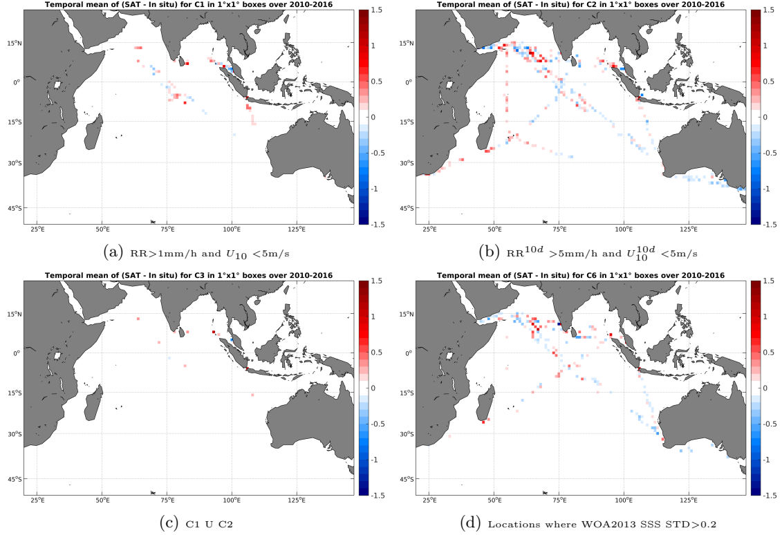
Figure 12: Temporal mean gridded over spatial boxes of size 1^\circ \times 1^\circ of \Delta SSS (SMOS-L3-CATDS-CECOS-LOCEAN-V2-18DAYS-25KM - TSG-LEGOS-DM) for 4 different subdatasets corresponding to: RR > 1\text{mm/h} and U_{10} < 5\text{m/s} (a), RR^{10d} > 5\text{mm/h} and U_{10}^{10d} < 5\text{m/s} (b), C1 U C2 (c), Locations where WOA2013 SSS STD > 0.2 (d).
