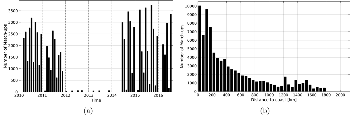
Figure 1: Number of match-ups between TSG-LEGOS-DM and SMOS-L3-CATDS-CECOS-LOCEAN-V2-18DAYS-25KM SSS as a function of time (a) and as function of the distance to coast (b) over the Indian Ocean Pi-MEP region and for the full satellite product period.
