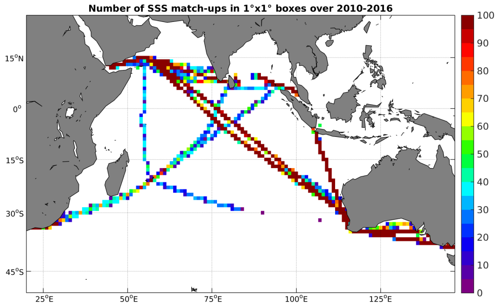
Figure 4: Number of SSS match-ups between TSG-LEGOS-DM SSS and the SMOS-L3-CATDS-CECOS-LOCEAN-V2-18DAYS-25KM SSS product for the Indian Ocean Pi-MEP region over 1°x1° boxes and for the full satellite product period.
