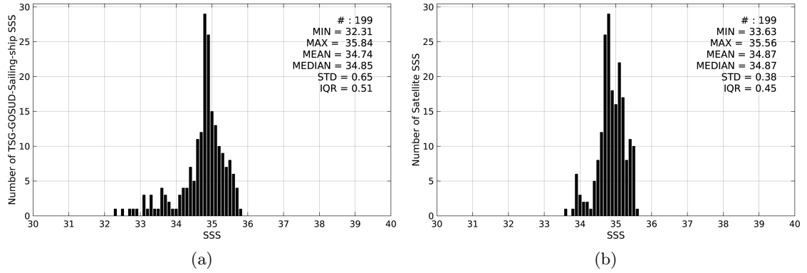
Figure 2: Histograms of SSS from TSG-GOSUD-Sailing-ship (a) and SMOS-L3-CATDS-CECOS-LOCEAN-V2-18DAYS-25KM (b) considering all match-up pairs per bins of 0.1 over the Indian Ocean Pi-MEP region and for the full satellite product period.
