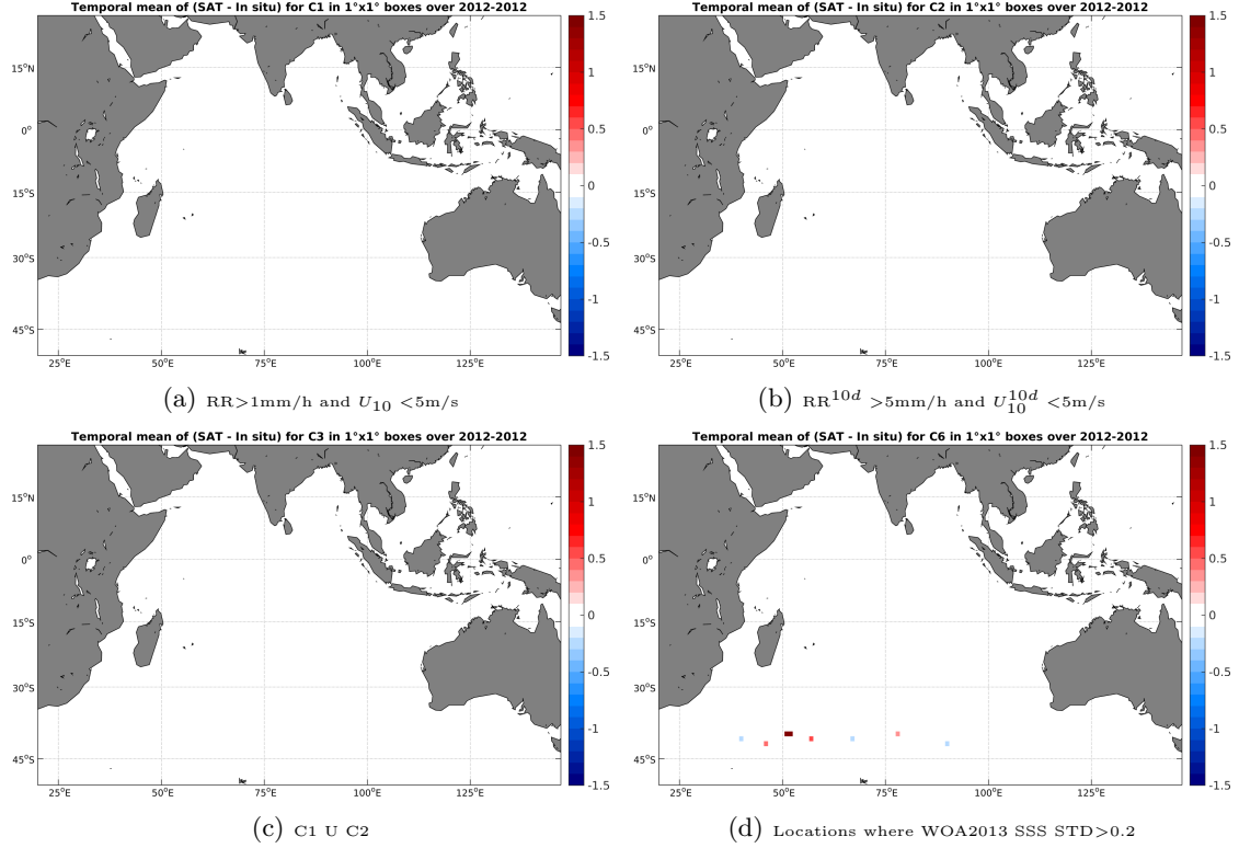
Figure 12: Temporal mean gridded over spatial boxes of size 1^\circ \times 1^\circ of \Delta SSS (SMOS-L3-CATDS-CECOS-LOCEAN-V2-18DAYS-25KM - TSG-GOSUD-Sailing-ship) for 4 different subdatasets corresponding to: RR > 1 mm/h and U_{10} < 5 m/s (a), RR^{10d} > 5 mm/h and U_{10}^{10d} < 5 m/s (b), C1 U C2 (c), Locations where WOA2013 SSS STD > 0.2 (d).
