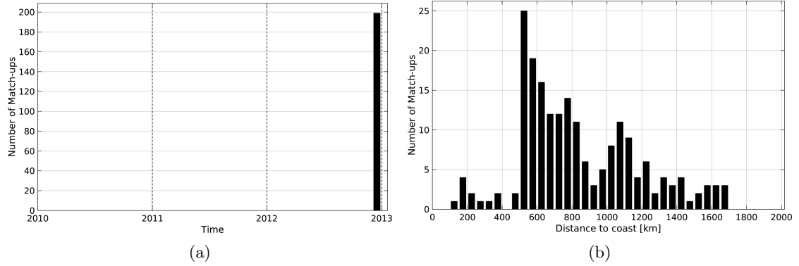
Figure 1: Number of match-ups between TSG-GOSUD-Sailing-ship and SMOS-L3-CATDS-CECOS-LOCEAN-V2-18DAYS-25KM SSS as a function of time (a) and as function of the distance to coast (b) over the Indian Ocean Pi-MEP region and for the full satellite product period.
