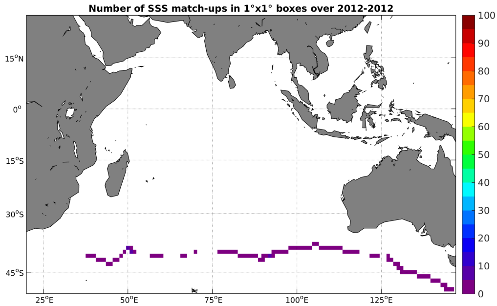
Figure 4: Number of SSS match-ups between TSG-GOSUD-Sailing-ship SSS and the SMOS-L3-CATDS-CECOS-LOCEAN-V2-18DAYS-25KM SSS product for the Indian Ocean Pi-MEP region over 1^\circ \times 1^\circ boxes and for the full satellite product period.
