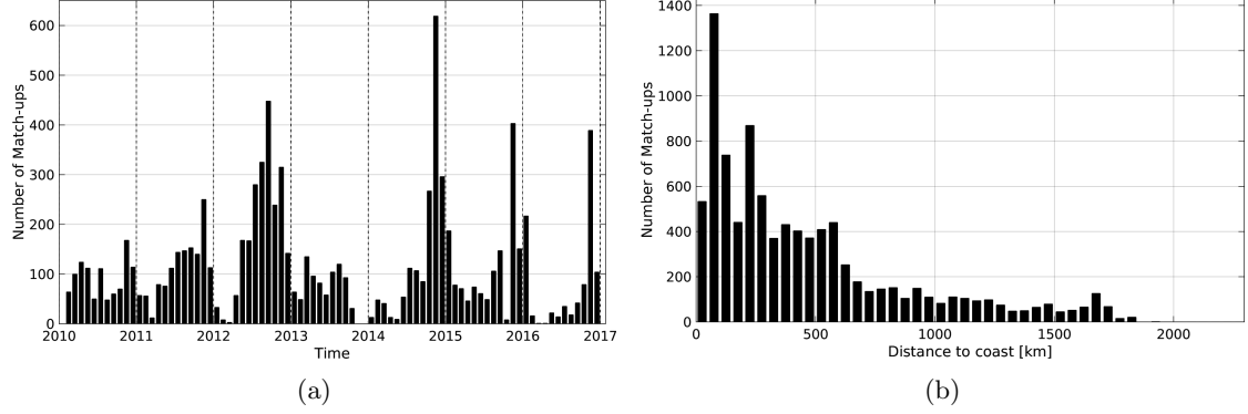
Figure 1: Number of match-ups between Sea mammals and SMOS-L3-CATDS-CECOS-LOCEAN-V2-18DAYS-25KM SSS as a function of time (a) and as function of the distance to coast (b) over the Indian Ocean Pi-MEP region and for the full satellite product period.
