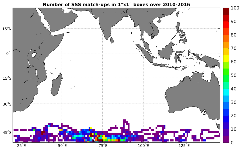
Figure 4: Number of SSS match-ups between Sea mammals SSS and the SMOS-L3-CATDS-CECOS-LOCEAN-V2-18DAYS-25KM SSS product for the Indian Ocean Pi-MEP region over 1^\circ \times 1^\circ boxes and for the full satellite product period.
