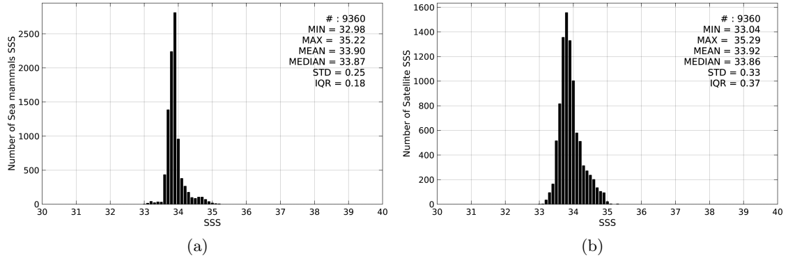
Figure 2: Histograms of SSS from Sea mammals (a) and SMOS-L3-CATDS-CECOS-LOCEAN-V2-18DAYS-25KM (b) considering all match-up pairs per bins of 0.1 over the Indian Ocean Pi-MEP region and for the full satellite product period.
