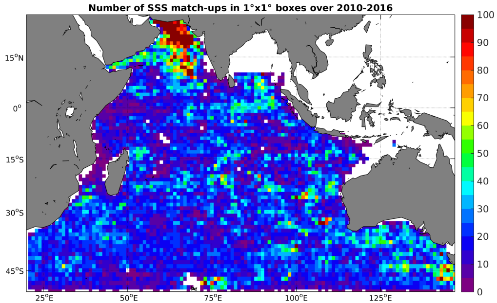
Figure 4: Number of SSS match-ups between Argo SSS and the SMOS-L3-CATDS-CECOS-LOCEAN-V2-18DAYS-25KM SSS product for the Indian Ocean Pi-MEP region over 1^\circ \times 1^\circ boxes and for the full satellite product period.
