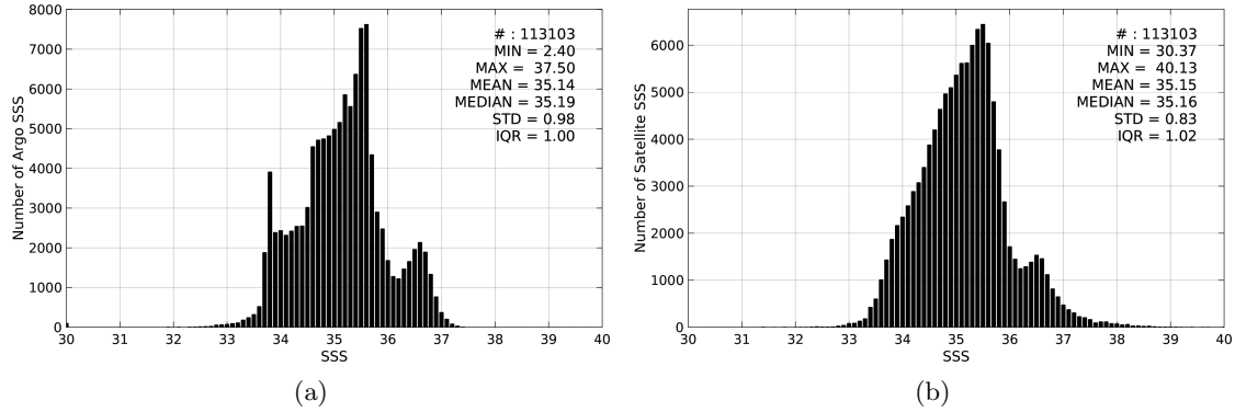
Figure 2: Histograms of SSS from Argo (a) and SMOS-L3-CATDS-CECOS-LOCEAN-V2-18DAYS-25KM (b) considering all match-up pairs per bins of 0.1 over the Indian Ocean Pi-MEP region and for the full satellite product period.
