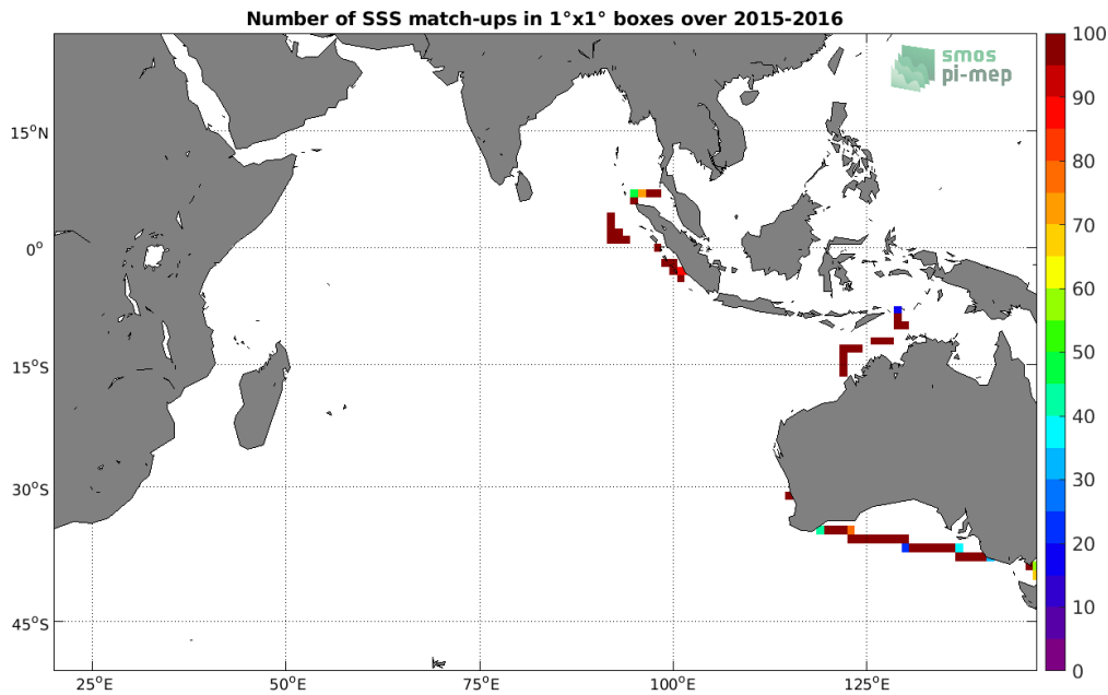
Figure 4: Number of SSS match-ups between TSG (SAMOS) SSS and the SMOS SSS L3 v2 - Monthly - 0.25 Deg (CATDS-CECOS-IFREMER) SSS product for the Indian Ocean Pi-MEP region over 1°x1° boxes and for the full satellite product period.
