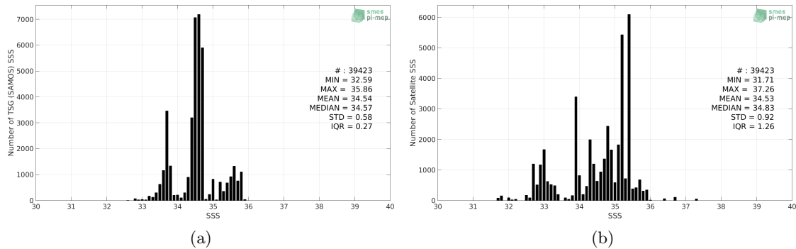
Figure 2: Histograms of SSS from TSG (SAMOS) (a) and SMOS SSS L3 v2 - Monthly - 0.25 Deg (CATDS-CECOS-IFREMER) (b) considering all match-up pairs per bins of 0.1 over the Indian Ocean Pi-MEP region and for the full satellite product period.
