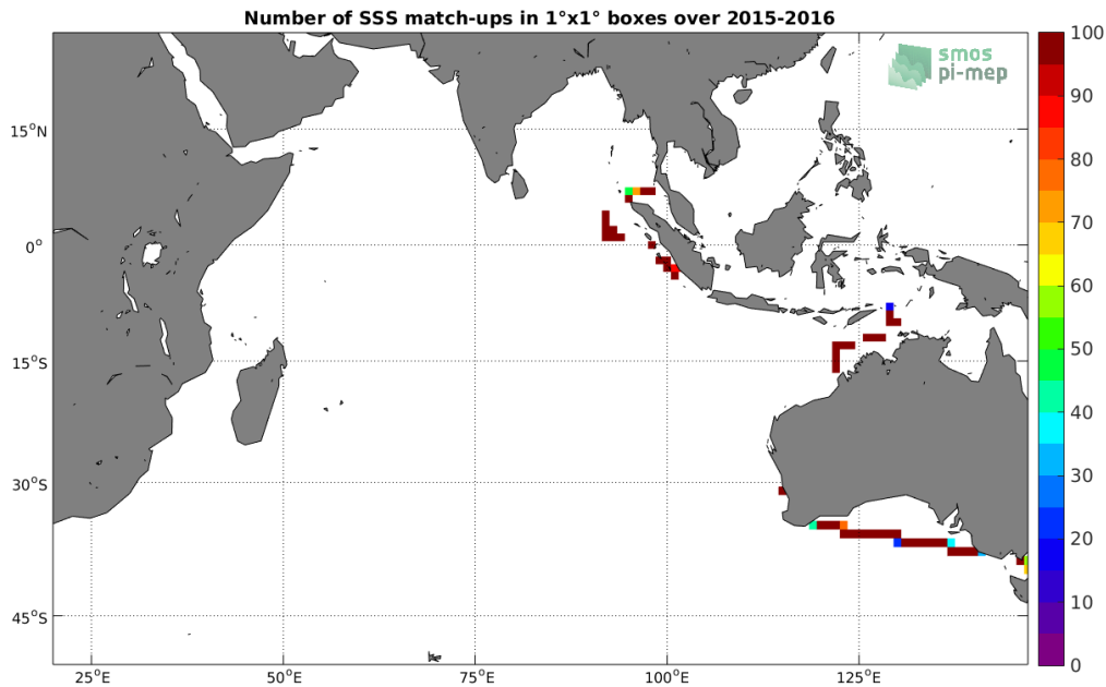
Figure 4: Number of SSS match-ups between TSG (SAMOS) SSS and the SMOS SSS L3 v2 - Monthly - 0.25 Deg (CATDS-CECOS-IFREMER) SSS product for the Indian Ocean Pi-MEP region over 1^\circ \times 1^\circ boxes and for the full satellite product period.
