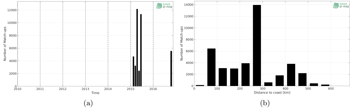
Figure 1: Number of match-ups between TSG (SAMOS) and SMOS SSS L3 v2 - Monthly - 0.25 Deg (CATDS-CECOS-IFREMER) SSS as a function of time (a) and as function of the distance to coast (b) over the Indian Ocean Pi-MEP region and for the full satellite product period.
