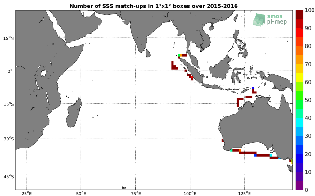
Figure 4: Number of SSS match-ups between TSG-SAMOS SSS and the SMOS L3 v2 - Monthly - 0.25 Deg (CATDS-CECOS-IFREMER) SSS product for the Indian Ocean Pi-MEP region over 1^\circ \times 1^\circ boxes and for the full satellite product period.
