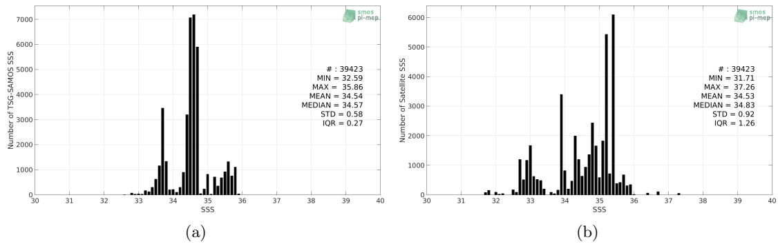
Figure 2: Histograms of SSS from TSG-SAMOS (a) and SMOS L3 v2 - Monthly - 0.25 Deg (CATDS-CECOS-IFREMER) (b) considering all match-up pairs per bins of 0.1 over the Indian Ocean Pi-MEP region and for the full satellite product period.
