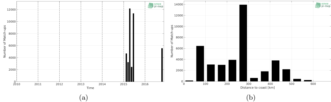
Figure 1: Number of match-ups between TSG-SAMOS and SMOS L3 v2 - Monthly - 0.25 Deg (CATDS-CECOS-IFREMER) SSS as a function of time (a) and as function of the distance to coast (b) over the Indian Ocean Pi-MEP region and for the full satellite product period.
