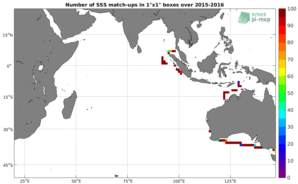
Figure 4: Number of SSS match-ups between TSG-SAMOS SSS and the SMOS-L3-CATDS-IFREMER-CECOS-V2-MONTHLY-0.25DEG SSS product for the Indian Ocean Pi-MEP region over 1^\circ \times 1^\circ boxes and for the full satellite product period.
