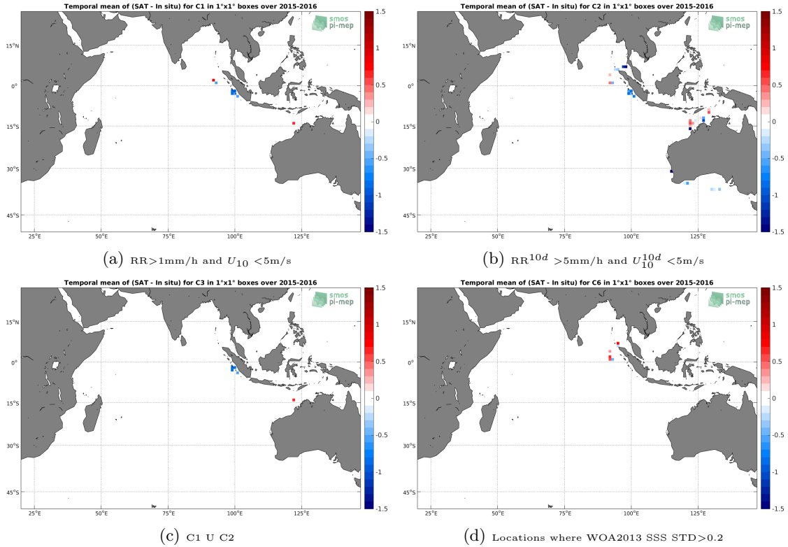
Figure 12: Temporal mean gridded over spatial boxes of size 1^\circ \times 1^\circ of \Delta SSS (SMOS-L3-CATDS-IFREMER-CECOS-V2-MONTHLY-0.25DEG - TSG-SAMOS) for 4 different subdatasets corresponding to:RR >1 mm/h and U_{10} < 5 m/s (a), RR 10d > 5 mm/h and U_{10}^{10d} < 5 m/s (b), C1 U C2 (c),Locations where WOA2013 SSS STD >0.2 (d).
