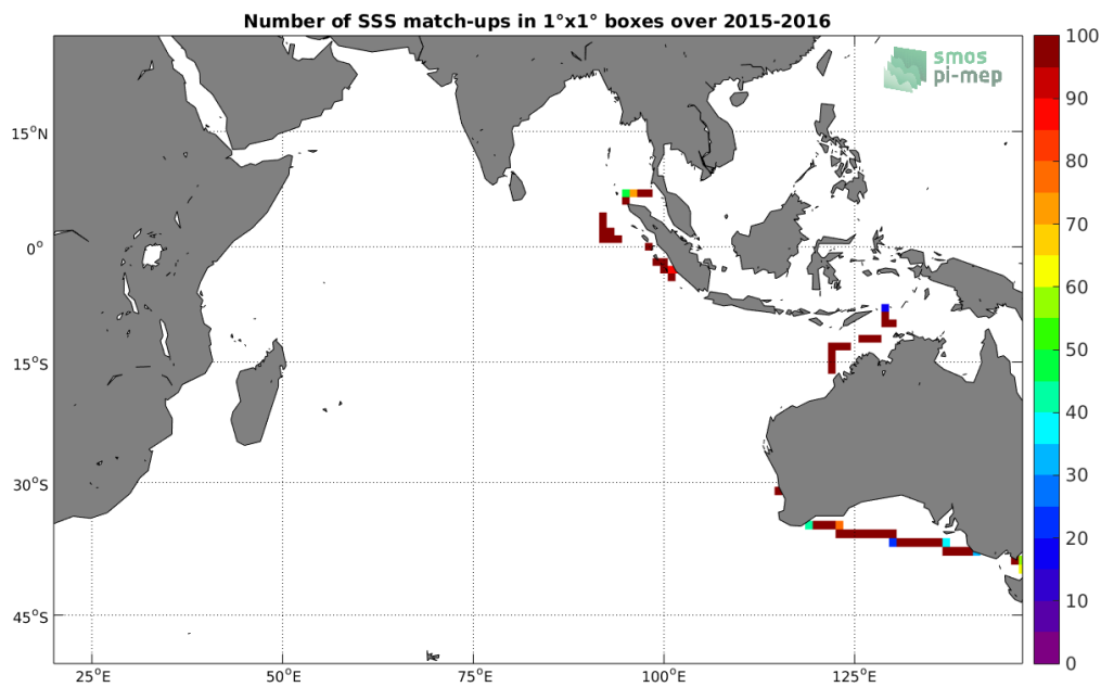
Figure 4: Number of SSS match-ups between TSG-SAMOS SSS and the SMOS-L3-CATDS-IFREMER-CECOS-V2-MONTHLY-0.25DEG SSS product for the Indian Ocean Pi-MEP region over 1^\circ \times 1^\circ boxes and for the full satellite product period.
