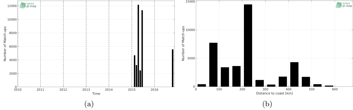
Figure 1: Number of match-ups between TSG-SAMOS and SMOS-L3-CATDS-IFREMER-CECOS-V2-MONTHLY-0.25DEG SSS as a function of time (a) and as function of the distance to coast (b) over the Indian Ocean Pi-MEP region and for the full satellite product period.
