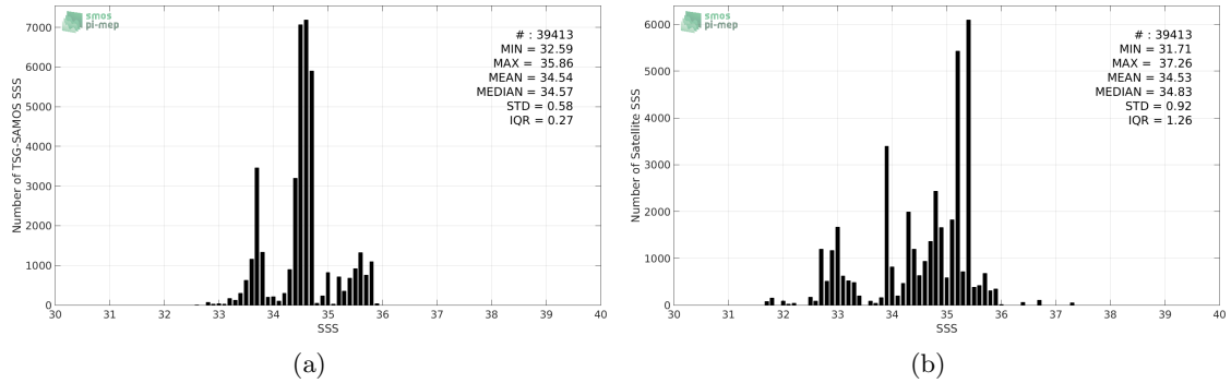
Figure 2: Histograms of SSS from TSG-SAMOS (a) and SMOS-L3-CATDS-IFREMER-CECOS-V2-MONTHLY-0.25DEG (b) considering all match-up pairs per bins of 0.1 over the Indian Ocean Pi-MEP region and for the full satellite product period.
