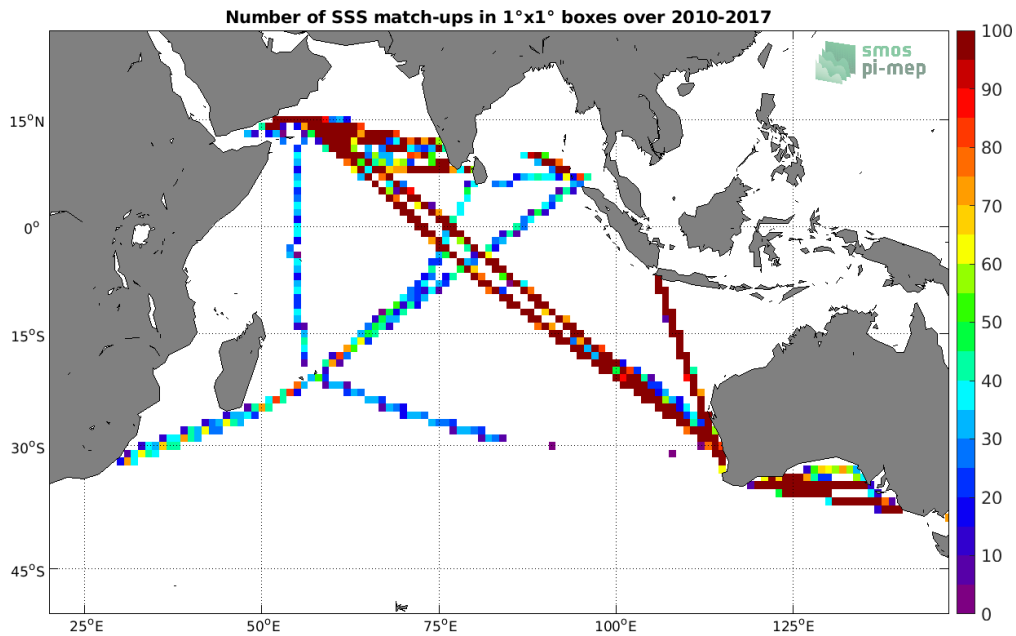
Figure 4: Number of SSS match-ups between TSG (LEGOS-DM) SSS and the SMOS SSS L3 v2 - Monthly - 0.25 Deg (CATDS-CECOS-IFREMER) SSS product for the Indian Ocean Pi-MEP region over 1^\circ \times 1^\circ boxes and for the full satellite product period.
