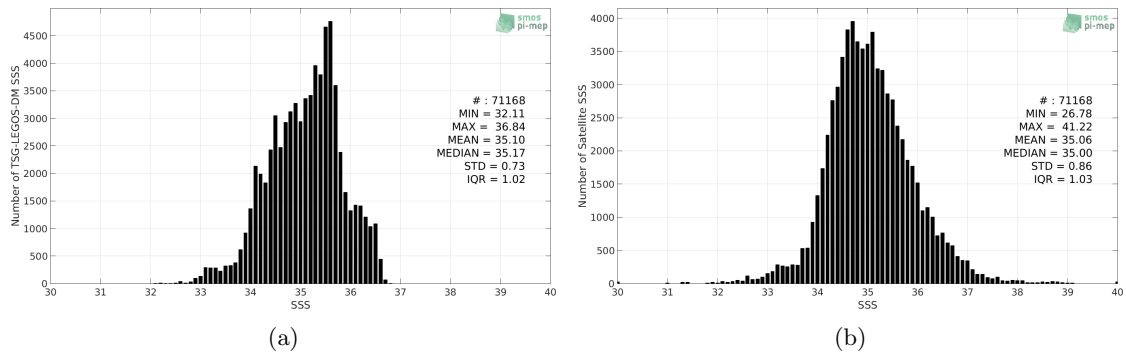
Figure 2: Histograms of SSS from TSG-LEGOS-DM (a) and SMOS L3 v2 - Monthly - 0.25 Deg (CATDS-CECOS-IFREMER) (b) considering all match-up pairs per bins of 0.1 over the Indian Ocean Pi-MEP region and for the full satellite product period.
