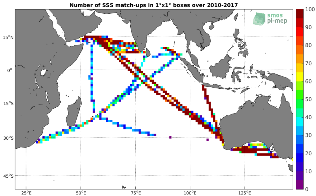
Figure 4: Number of SSS match-ups between TSG-LEGOS-DM SSS and the SMOS L3 v2 - Monthly - 0.25 Deg (CATDS-CECOS-IFREMER) SSS product for the Indian Ocean Pi-MEP region over 1°x1° boxes and for the full satellite product period.
