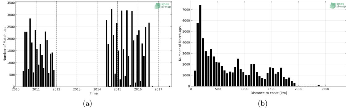
Figure 1: Number of match-ups between TSG-LEGOS-DM and SMOS L3 v2 - Monthly - 0.25 Deg (CATDS-CECOS-IFREMER) SSS as a function of time (a) and as function of the distance to coast (b) over the Indian Ocean Pi-MEP region and for the full satellite product period.
