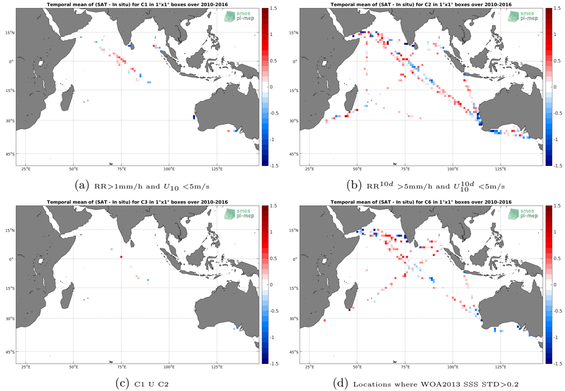
Figure 12: Temporal mean gridded over spatial boxes of size 1^\circ \times 1^\circ of \Delta\text{SSS} (SMOS-L3-CATDS-IFREMER-CECOS-V2-MONTHLY-0.25DEG - TSG-LEGOS-DM) for 4 different subdatasets corresponding to: RR > 1mm/h and U_{10} < 5\text{m/s} (a), RR^{10d} > 5\text{mm/h} and U_{10}^{10d} < 5\text{m/s} (b), C1 U C2 (c), Locations where WOA2013 SSS STD > 0.2 (d).
