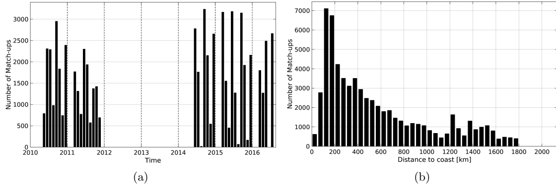
Figure 1: Number of match-ups between TSG-LEGOS-DM and SMOS-L3-CATDS-IFREMER-CECOS-V2-MONTHLY-0.25DEG SSS as a function of time (a) and as function of the distance to coast (b) over the Indian Ocean Pi-MEP region and for the full satellite product period.
