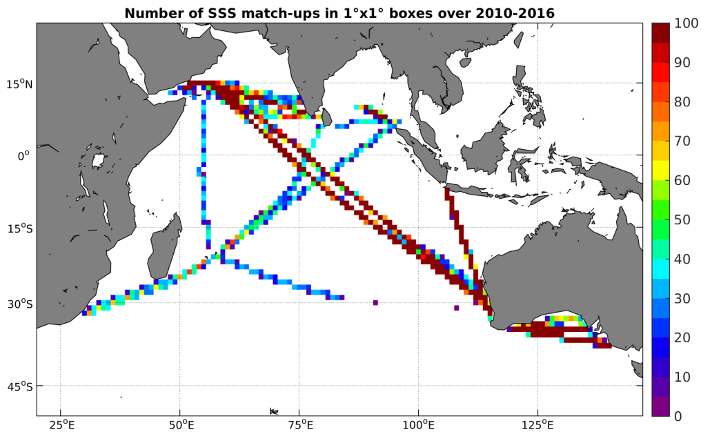
Figure 4: Number of SSS match-ups between TSG-LEGOS-DM SSS and the SMOS-L3-CATDS-IFREMER-CECOS-V2-MONTHLY-0.25DEG SSS product for the Indian Ocean Pi-MEP region over 1^\circ \times 1^\circ boxes and for the full satellite product period.
