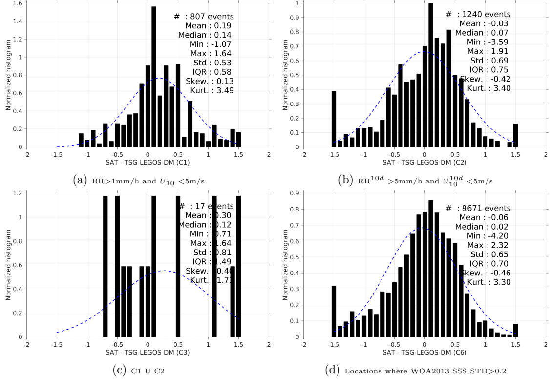
Figure 13: Normalized histogram of \Delta SSS (SMOS-L3-CATDS-IFREMER-CECOS-V2-MONTHLY-0.25DEG - TSG-LEGOS-DM) for 6 different subdatasets corresponding to: RR > 1mm/h and U_{10} < 5 m/s (a), RR^{10d} > 5 mm/h and U_{10}^{10d} < 5 m/s (b), C1 U C2 (c), Locations where WOA2013 SSS STD > 0.2 (d).
