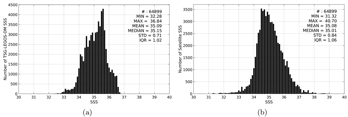
Figure 2: Histograms of SSS from TSG-LEGOS-DM (a) and SMOS-L3-CATDS-IFREMER-CECOS-V2-MONTHLY-0.25DEG (b) considering all match-up pairs per bins of 0.1 over the Indian Ocean Pi-MEP region and for the full satellite product period.
