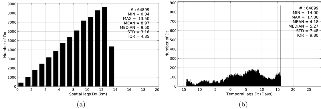
Figure 5: Histograms of the spatial (a) and temporal (b) lags between the time of the TSG-LEGOS-DM measurements and the date of the corresponding SMOS-L3-CATDS-IFREMER-CECOS-V2-MONTHLY-0.25DEG SSS product.
