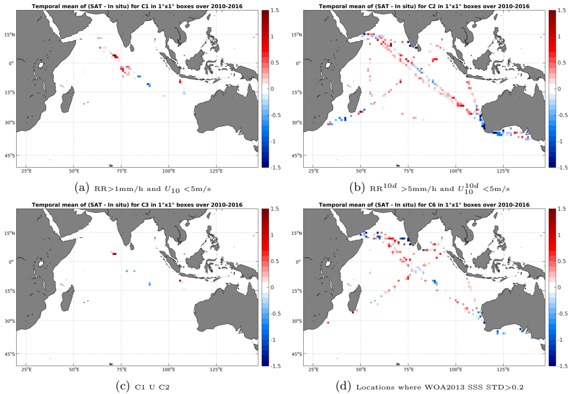
Figure 12: Temporal mean gridded over spatial boxes of size 1^\circ \times 1^\circ of \Delta SSS (SMOS-L3-CATDS-IFREMER-CECOS-V2-MONTHLY-0.25DEG - TSG-LEGOS-DM) for 4 different subdatasets corresponding to: RR > 1\text{mm/h} and U_{10} < 5\text{m/s} (a), RR^{10d} > 5\text{mm/h} and U_{10}^{10d} < 5\text{m/s} (b), C1 U C2 (c), Locations where WOA2013 SSS STD > 0.2 (d).
