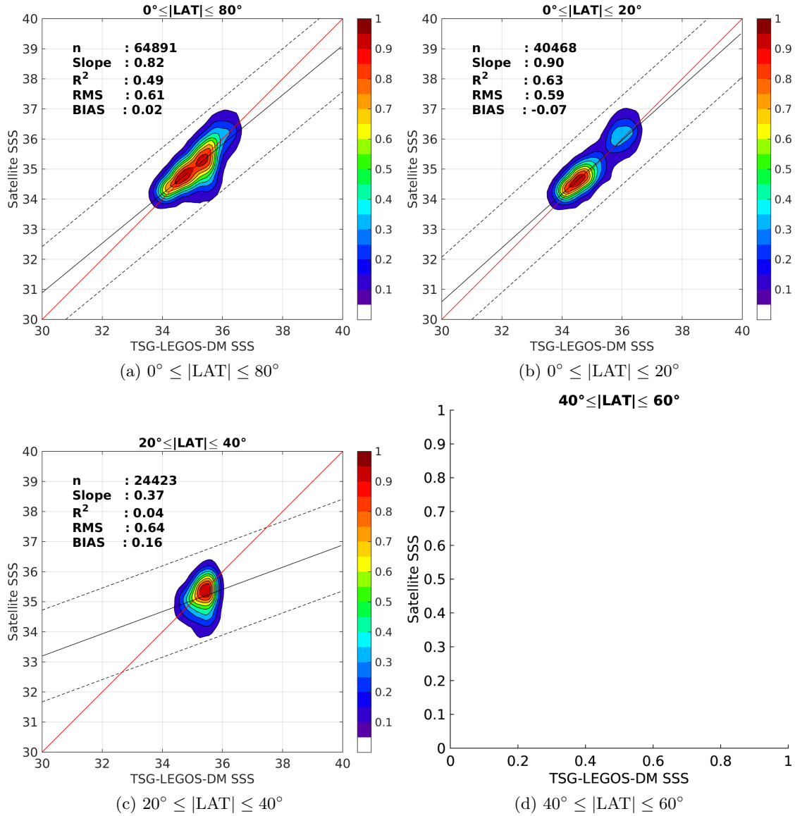
Figure 9: Contour maps of the concentration of SMOS-L3-CATDS-IFREMER-CECOS-V2-MONTHLY-0.25DEG SSS ( y -axis) versus TSG-LEGOS-DM SSS ( x -axis) at match-up pairs for different latitude bands. For each plot, the red line shows x=y . The black thin and dashed lines indicate a linear fit through the data cloud and the \pm 95\% confidence levels, respectively. The number match-up pairs n , the slope and R^2 coefficient of the linear fit, the root mean square (RMS) and the mean bias between satellite and in situ data are indicated for each latitude band in each plots.
