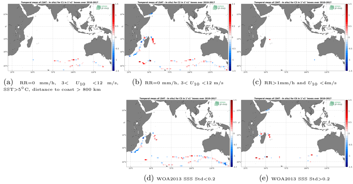
Figure 12: Temporal mean gridded over spatial boxes of size 1^\circ \times 1^\circ of \Delta SSS (SMOS SSS L3 v2 - Monthly - 0.25 Deg (CATDS-CECOS-IFREMER) - TSG (GOSUD-Sailing-ship)) for 5 different subdatasets corresponding to:RR=0 mm/h, 3 < U_{10} < 12 m/s, SST >5^\circ C, distance to coast > 800 km (a), RR=0 mm/h, 3 < U_{10} < 12 m/s (b), RR >1 mm/h and U_{10} < 4 m/s (c), WOA2013 SSS Std <0.2 (d), WOA2013 SSS Std >0.2 (e).
