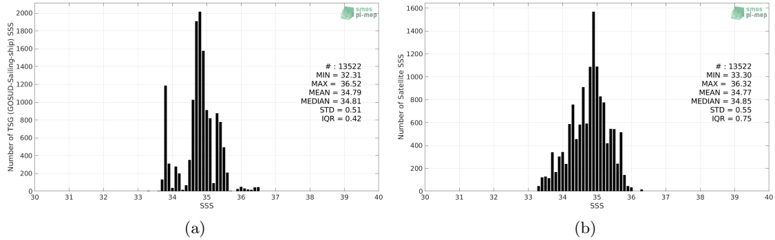
Figure 2: Histograms of SSS from TSG (GOSUD-Sailing-ship) (a) and SMOS SSS L3 v2 - Monthly - 0.25 Deg (CATDS-CECOS-IFREMER) (b) considering all match-up pairs per bins of 0.1 over the Indian Ocean Pi-MEP region and for the full satellite product period.
