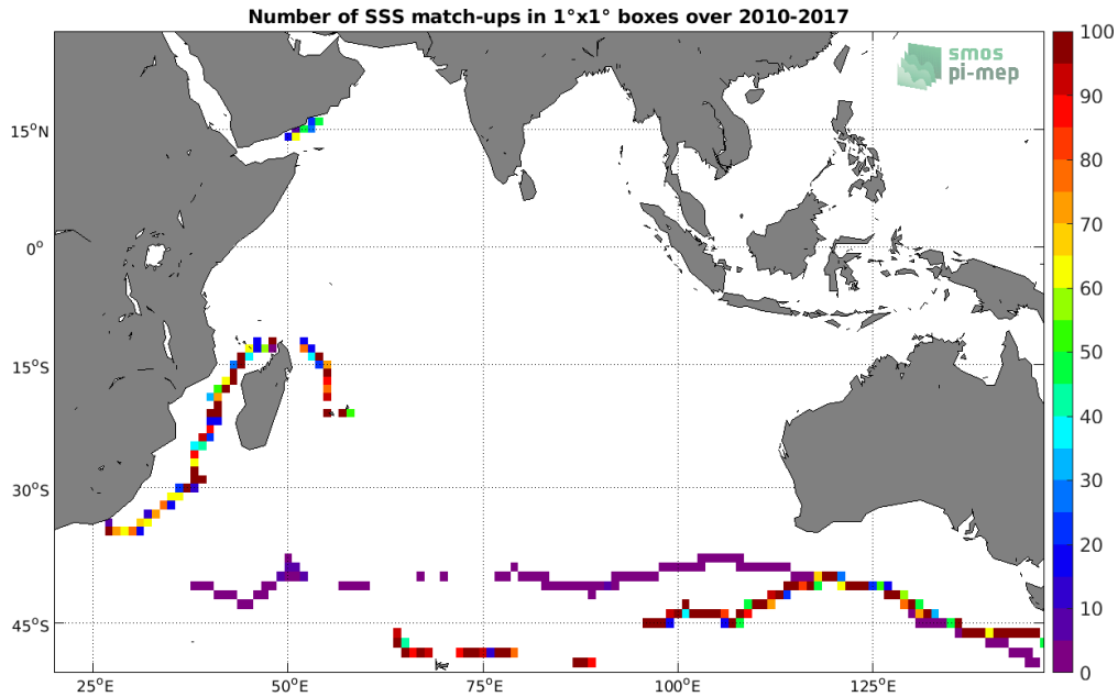
Figure 4: Number of SSS match-ups between TSG (GOSUD-Sailing-ship) SSS and the SMOS SSS L3 v2 - Monthly - 0.25 Deg (CATDS-CECOS-IFREMER) SSS product for the Indian Ocean Pi-MEP region over 1^\circ \times 1^\circ boxes and for the full satellite product period.
