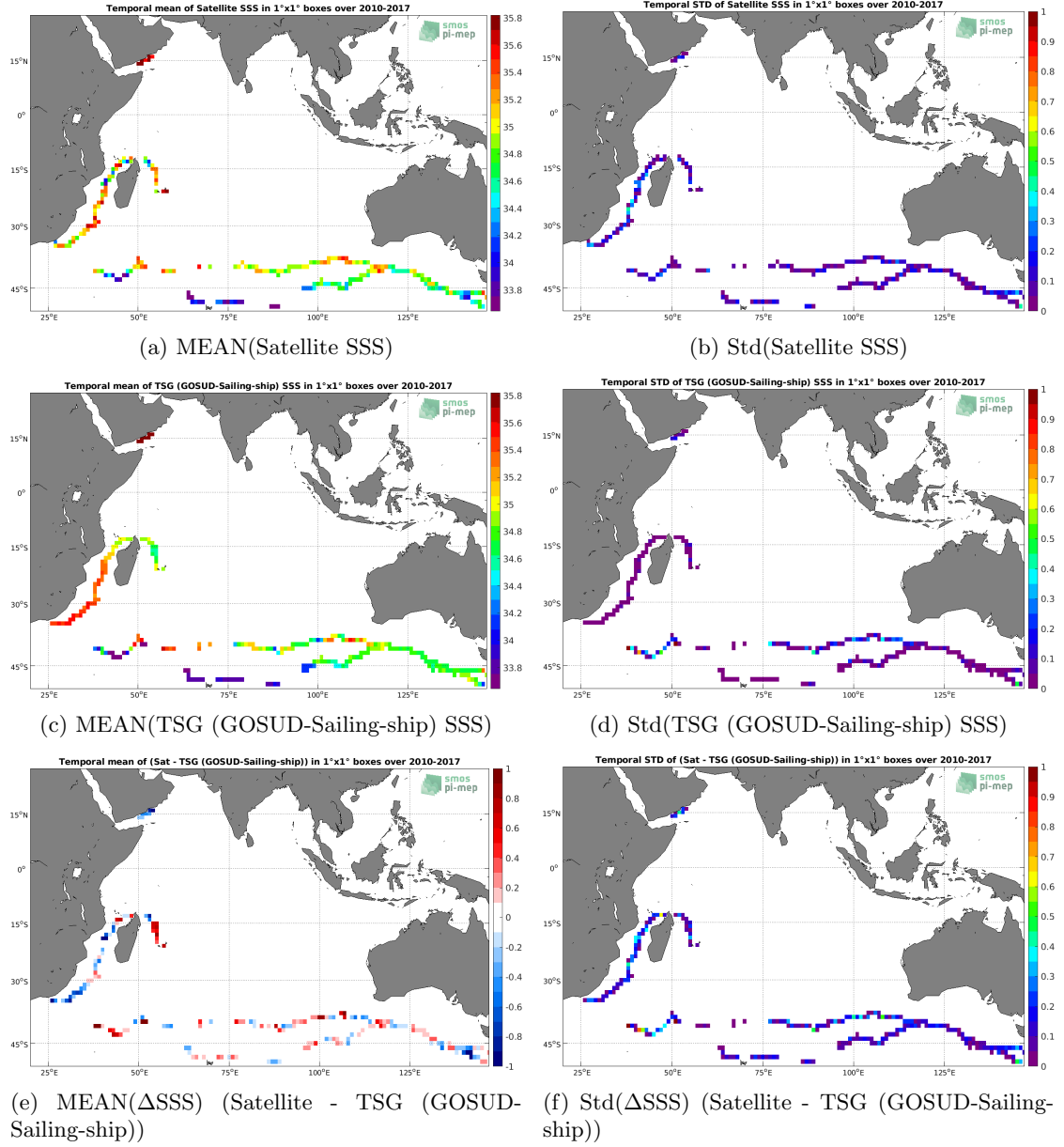
Figure 6: Temporal mean (left) and Std (right) of SSS from SMOS SSS L3 v2 - Monthly - 0.25 Deg (CATDS-CECOS-IFREMER) (top), TSG (GOSUD-Sailing-ship) (middle), and of \Delta SSS (Satellite - TSG (GOSUD-Sailing-ship)). Only match-up pairs are used to generate these maps.
