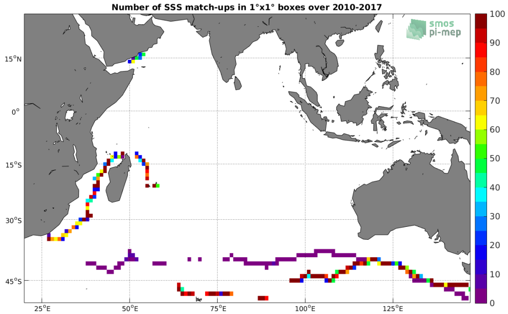
Figure 4: Number of SSS match-ups between TSG (GOSUD-Sailing-ship) SSS and the SMOS SSS L3 v2 - Monthly - 0.25 Deg (CATDS-CECOS-IFREMER) SSS product for the Indian Ocean Pi-MEP region over 1°x1° boxes and for the full satellite product period.
