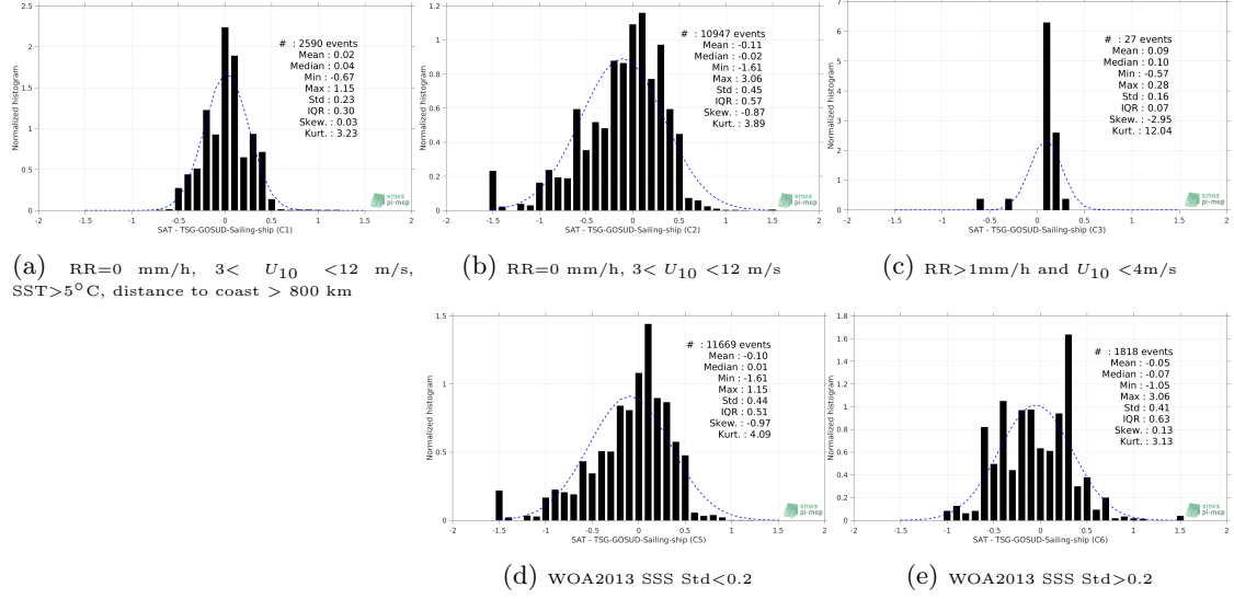
Figure 13: Normalized histogram of \Delta\text{SSS} (SMOS L3 v2 - Monthly - 0.25 Deg (CATDS-CECOS-IFREMER) - TSG-GOSUD-Sailing-ship) for 5 different subdatasets corresponding to: RR=0 mm/h, 3 < U_{10} < 12 m/s, SST > 5^\circ\text{C} , distance to coast > 800 km (a), RR=0 mm/h, 3 < U_{10} < 12 m/s (b), RR > 1\text{mm/h} and U_{10} < 4\text{m/s} (c), WOA2013 SSS Std < 0.2 (d), WOA2013 SSS Std > 0.2 (e).
