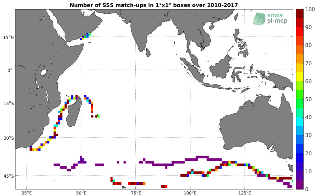
Figure 4: Number of SSS match-ups between TSG-GOSUD-Sailing-ship SSS and the SMOS L3 v2 - Monthly - 0.25 Deg (CATDS-CECOS-IFREMER) SSS product for the Indian Ocean Pi-MEP region over 1°x1° boxes and for the full satellite product period.
