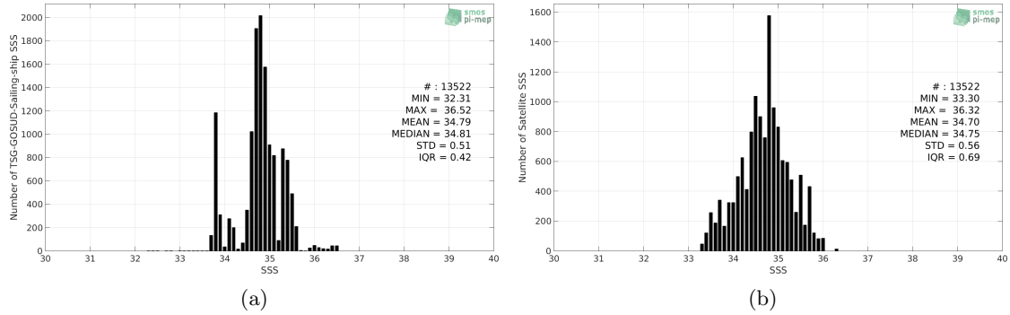
Figure 2: Histograms of SSS from TSG-GOSUD-Sailing-ship (a) and SMOS L3 v2 - Monthly - 0.25 Deg (CATDS-CECOS-IFREMER) (b) considering all match-up pairs per bins of 0.1 over the Indian Ocean Pi-MEP region and for the full satellite product period.
