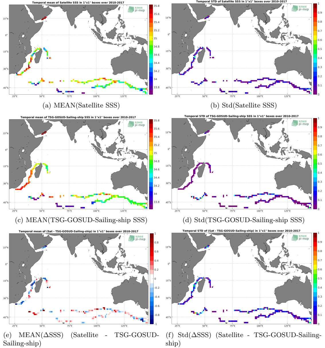
Figure 6: Temporal mean (left) and Std (right) of SSS from SMOS L3 v2 - Monthly - 0.25 Deg (CATDS-CECOS-IFREMER) (top), TSG-GOSUD-Sailing-ship (middle), and of \Delta SSS (Satellite - TSG-GOSUD-Sailing-ship). Only match-up pairs are used to generate these maps.
