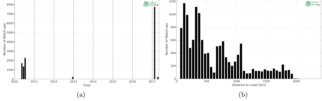
Figure 1: Number of match-ups between TSG-GOSUD-Sailing-ship and SMOS-L3-CATDS-IFREMER-CECOS-V2-MONTHLY-0.25DEG SSS as a function of time (a) and as function of the distance to coast (b) over the Indian Ocean Pi-MEP region and for the full satellite product period.
