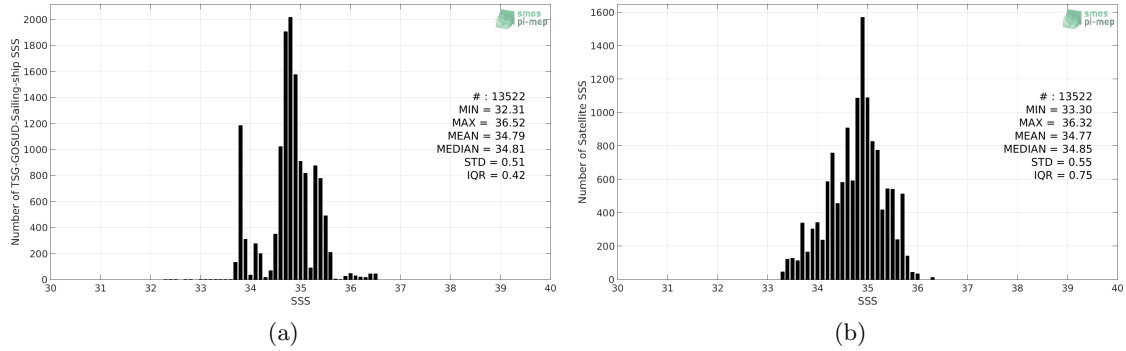
Figure 2: Histograms of SSS from TSG-GOSUD-Sailing-ship (a) and SMOS-L3-CATDS-IFREMER-CECOS-V2-MONTHLY-0.25DEG (b) considering all match-up pairs per bins of 0.1 over the Indian Ocean Pi-MEP region and for the full satellite product period.
