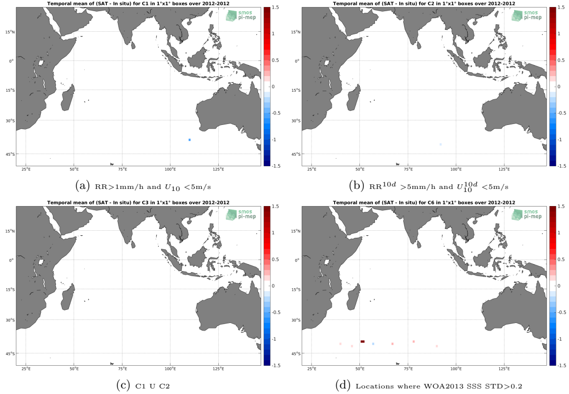
Figure 12: Temporal mean gridded over spatial boxes of size 1^\circ \times 1^\circ of \Delta SSS (SMOS-L3-CATDS-IFREMER-CECOS-V2-MONTHLY-0.25DEG - TSG-GOSUD-Sailing-ship) for 4 different sub-datasets corresponding to: RR > 1\text{mm/h} and U_{10} < 5\text{m/s} (a), RR^{10d} > 5\text{mm/h} and U_{10}^{10d} < 5\text{m/s} (b), C1 U C2 (c), Locations where WOA2013 SSS STD > 0.2 (d).
