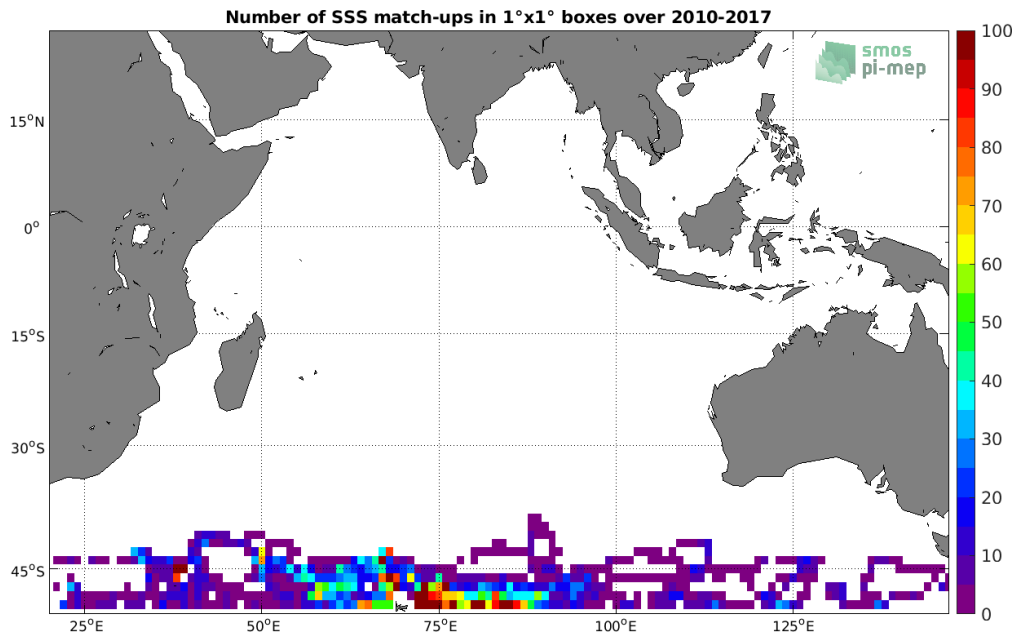
Figure 4: Number of SSS match-ups between Sea mammals SSS and the SMOS SSS L3 v2 - Monthly - 0.25 Deg (CATDS-CECOS-IFREMER) SSS product for the Indian Ocean Pi-MEP region over 1^\circ \times 1^\circ boxes and for the full satellite product period.
