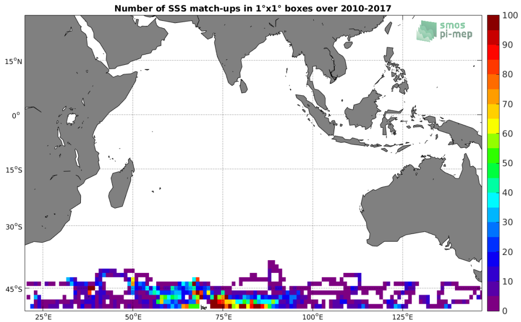
Figure 4: Number of SSS match-ups between Sea mammals SSS and the SMOS-L3-CATDS-IFREMER-CECOS-V2-MONTHLY-0.25DEG SSS product for the Indian Ocean Pi-MEP region over 1^{\circ} \times 1^{\circ} boxes and for the full satellite product period.
