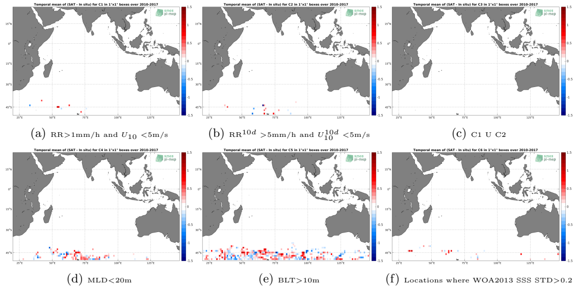
Figure 12: Temporal mean gridded over spatial boxes of size 1^\circ \times 1^\circ of \Delta\text{SSS} (SMOS-L3-CATDS-IFREMER-CECOS-V2-MONTHLY-0.25DEG - Sea mammals) for 6 different subdatasets corresponding to: \text{RR} > 1\text{mm/h} and U_{10} < 5\text{m/s} (a), \text{RR}^{10d} > 5\text{mm/h} and U_{10}^{10d} < 5\text{m/s} (b), C1 U C2 (c), \text{MLD} < 20\text{m} (d), \text{BLT} > 10\text{m} (e), Locations where WOA2013 SSS STD > 0.2 (f).
