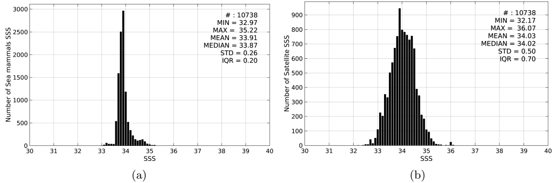
Figure 2: Histograms of SSS from Sea mammals (a) and SMOS-L3-CATDS-IFREMER-CECOS-V2-MONTHLY-0.25DEG (b) considering all match-up pairs per bins of 0.1 over the Indian Ocean Pi-MEP region and for the full satellite product period.
