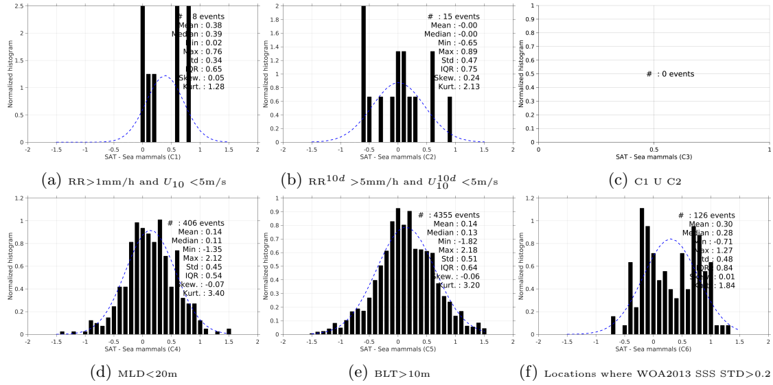
Figure 13: Normalized histogram of \Delta SSS (SMOS-L3-CATDS-IFREMER-CECOS-V2-MONTHLY-0.25DEG - Sea mammals) for 6 different subdatasets corresponding to: RR > 1mm/h and U_{10} < 5 m/s (a), RR 10d > 5mm/h and U_{10}^{10d} < 5 m/s (b), C1 U C2 (c), MLD < 20m (d), BLT > 10m (e), Locations where WOA2013 SSS STD > 0.2 (f).
