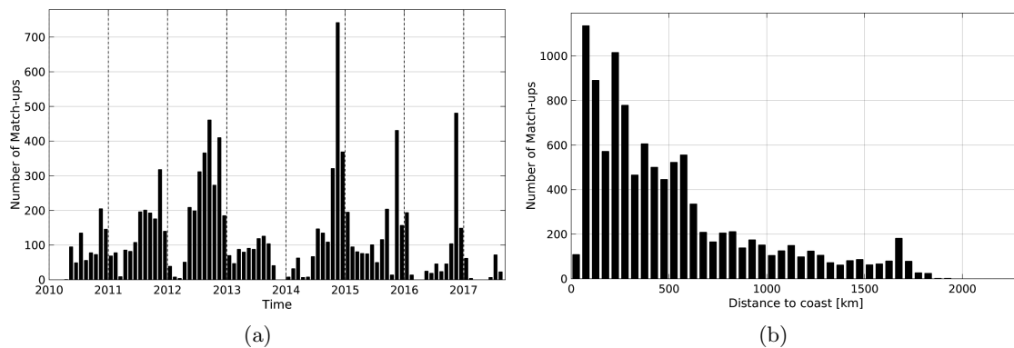
Figure 1: Number of match-ups between Sea mammals and SMOS-L3-CATDS-IFREMER-CECOS-V2-MONTHLY-0.25DEG SSS as a function of time (a) and as function of the distance to coast (b) over the Indian Ocean Pi-MEP region and for the full satellite product period.
