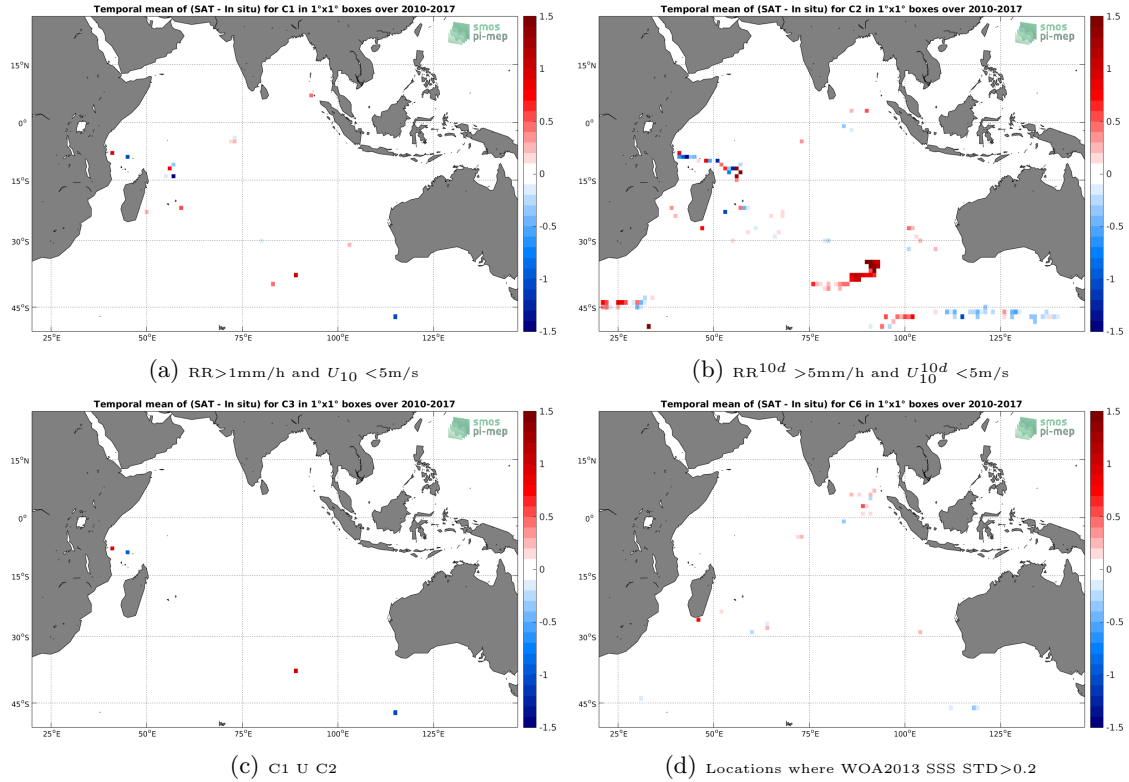
Figure 11: Temporal mean gridded over spatial boxes of size 1^\circ \times 1^\circ of \Delta SSS (SMOS-L3-CATDS-IFREMER-CECOS-V2-MONTHLY-0.25DEG - Surface drifters) for 4 different subdatasets corresponding to: RR > 1 mm/h and U_{10} < 5 m/s (a), RR 10d > 5 mm/h and U_{10}^{10d} < 5 m/s (b), C1 U C2 (c), Locations where WOA2013 SSS STD > 0.2 (d).
