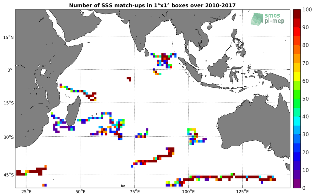
Figure 3: Number of SSS match-ups between Surface drifters SSS and the SMOS-L3-CATDS-IFREMER-CECOS-V2-MONTHLY-0.25DEG SSS product for the Indian Ocean Pi-MEP region over 1^\circ \times 1^\circ boxes and for the full satellite product period.
