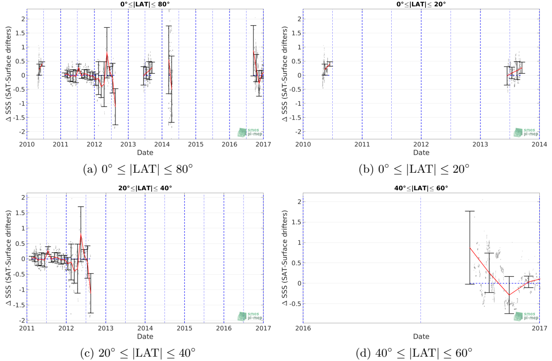
Figure 9: Monthly-average mean (red curves) \Delta SSS (Satellite - Surface drifters) and \pm 1 STD (black vertical thick bars) as function of time for all the collected Pi-MEP match-up pairs estimated over the Indian Ocean Pi-MEP region and for the full satellite product period are shown for different latitude bands: (a) Latitude band 80^\circ\text{S}-80^\circ\text{N} , (b) latitude band 20^\circ\text{S}-20^\circ\text{N} , (c) Mid Latitude bands 40^\circ\text{S}-20^\circ\text{S} and 20^\circ\text{N}-40^\circ\text{N} and (d) Latitude bands 60^\circ\text{S}-40^\circ\text{S} and 40^\circ\text{N}-60^\circ\text{N} .
