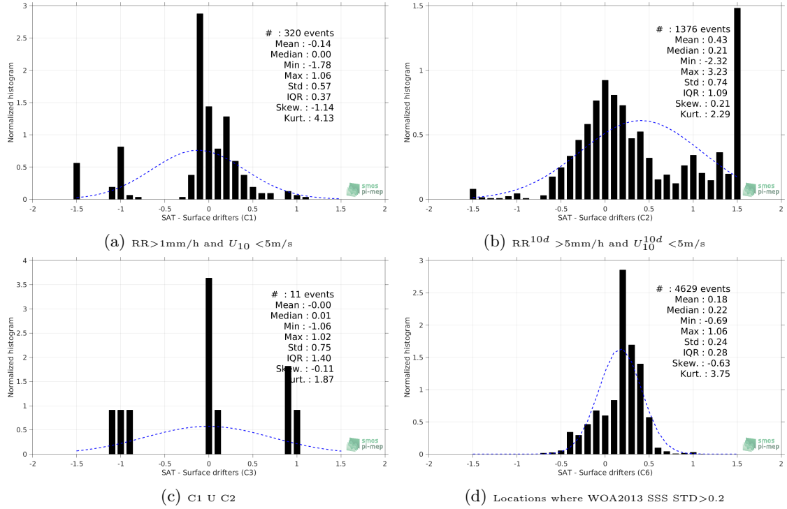
Figure 12: Normalized histogram of \Delta SSS (SMOS-L3-CATDS-IFREMER-CECOS-V2-MONTHLY-0.25DEG - Surface drifters) for 6 different subdatasets corresponding to: RR > 1\text{mm/h} and U_{10} < 5\text{m/s} (a), RR^{10d} > 5\text{mm/h} and U_{10}^{10d} < 5\text{m/s} (b), C1 \cup C2 (c), Locations where WOA2013 SSS STD > 0.2 (d).
