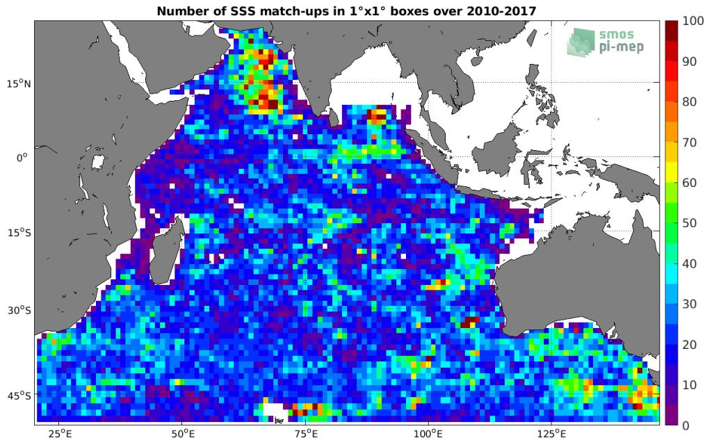
Figure 4: Number of SSS match-ups between Argo SSS and the SMOS SSS L3 v2 - Monthly - 0.25 Deg (CATDS-CECOS-IFREMER) SSS product for the Indian Ocean Pi-MEP region over 1^\circ \times 1^\circ boxes and for the full satellite product period.
