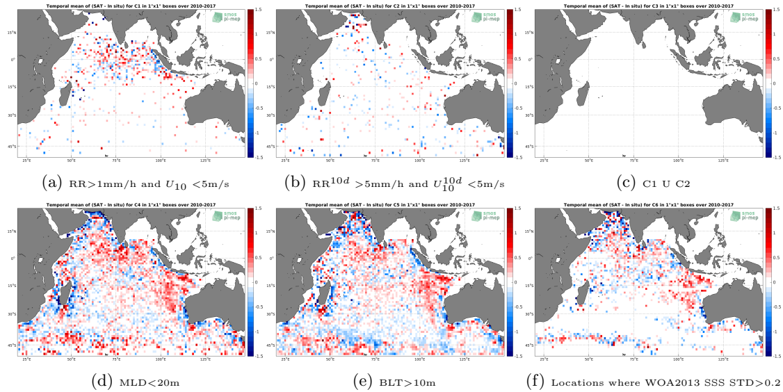
Figure 12: Temporal mean gridded over spatial boxes of size 1^\circ \times 1^\circ of \Delta\text{SSS} (SMOS-L3-CATDS-IFREMER-CECOS-V2-MONTHLY-0.25DEG - Argo) for 6 different subdatasets corresponding to: RR > 1\text{mm/h} and U_{10} < 5\text{m/s} (a), RR^{10d} > 5\text{mm/h} and U_{10}^{10d} < 5\text{m/s} (b), C1 U C2 (c), MLD < 20\text{m} (d), BLT > 10\text{m} (e), Locations where WOA2013 SSS STD > 0.2 (f).
