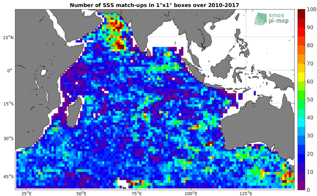
Figure 4: Number of SSS match-ups between Argo SSS and the SMOS-L3-CATDS-IFREMER-CECOS-V2-MONTHLY-0.25DEG SSS product for the Indian Ocean Pi-MEP region over 1°x1° boxes and for the full satellite product period.
